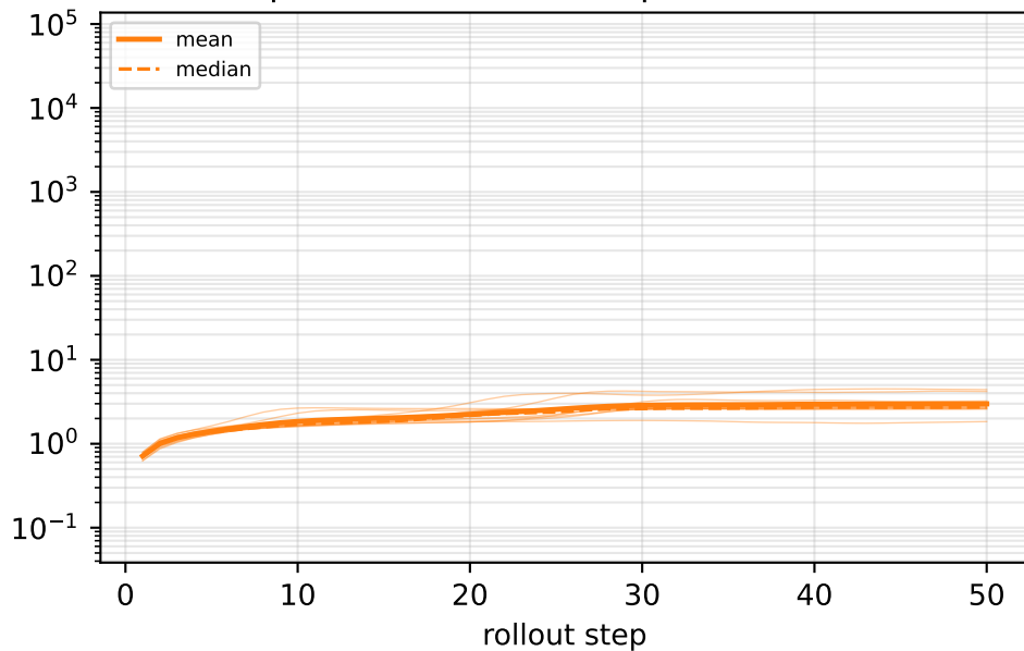
FNO MHD-pretrain zero-FT step1: 0.715 \pm 0.058 , step50: 2.99 \pm 0.74
