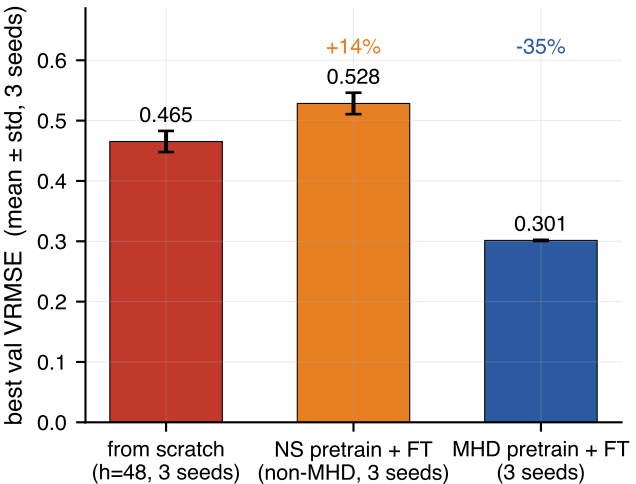
Matched-architecture transfer at 1% target data
