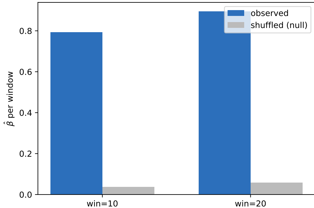
Drift rate: observed vs temporal-shuffle null
