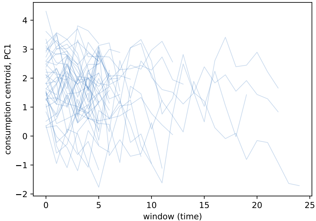
Per-user consumption trajectories (PC1, win=20)
