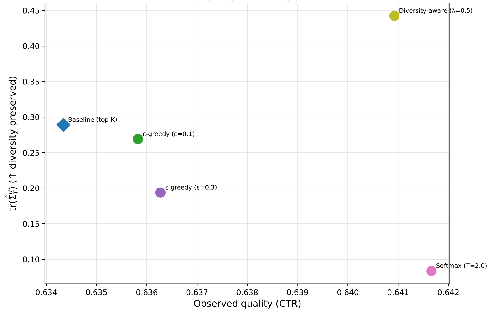
H5: Pareto — quality vs diversity preservation
