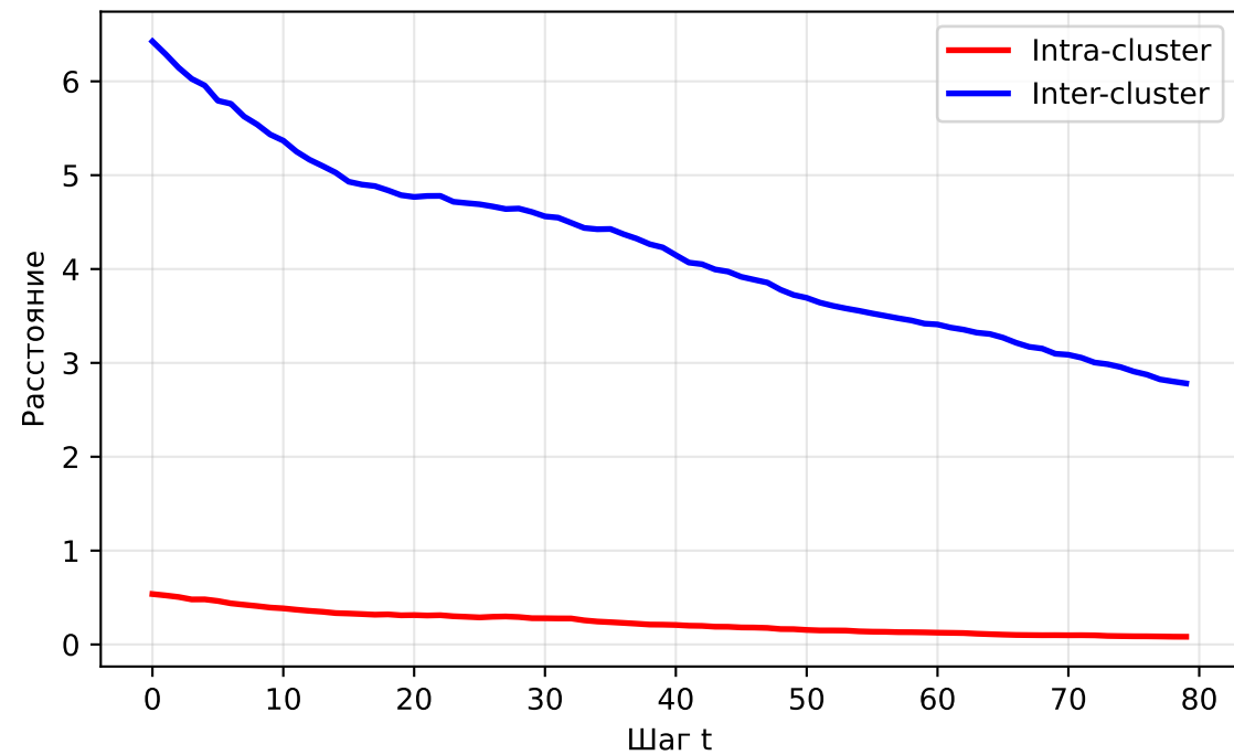
K=4: Inter vs Intra cluster distance
