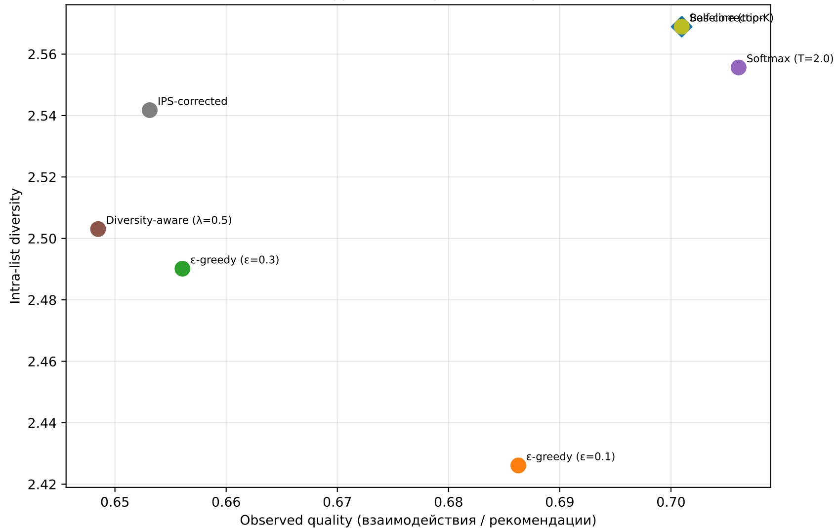
H5: Pareto-фронт Quality vs Diversity (t=70)
