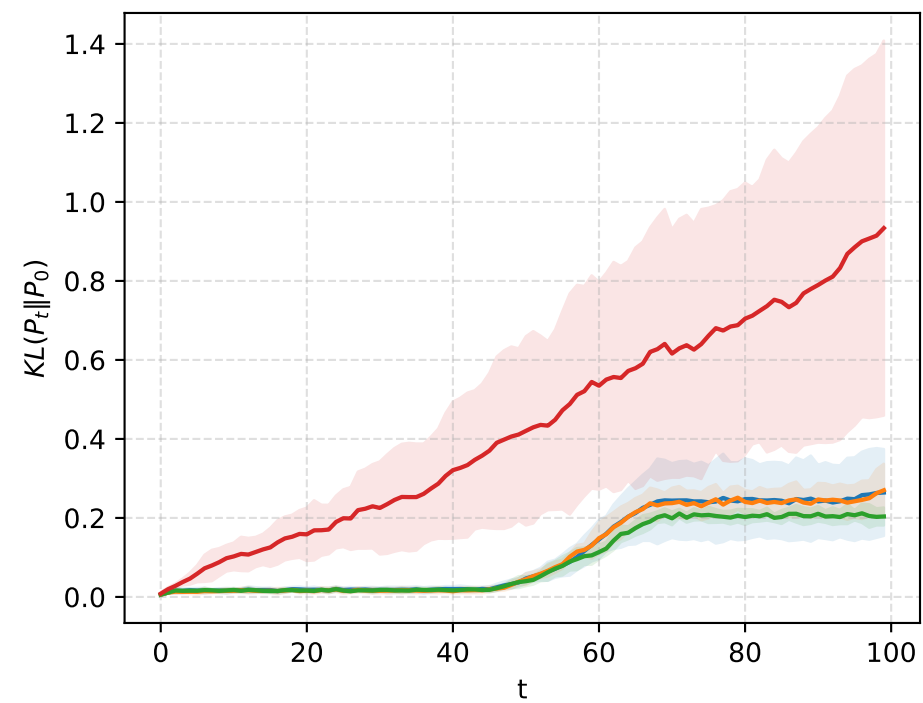
Mechanism diagnostic: \beta=0 контроли
