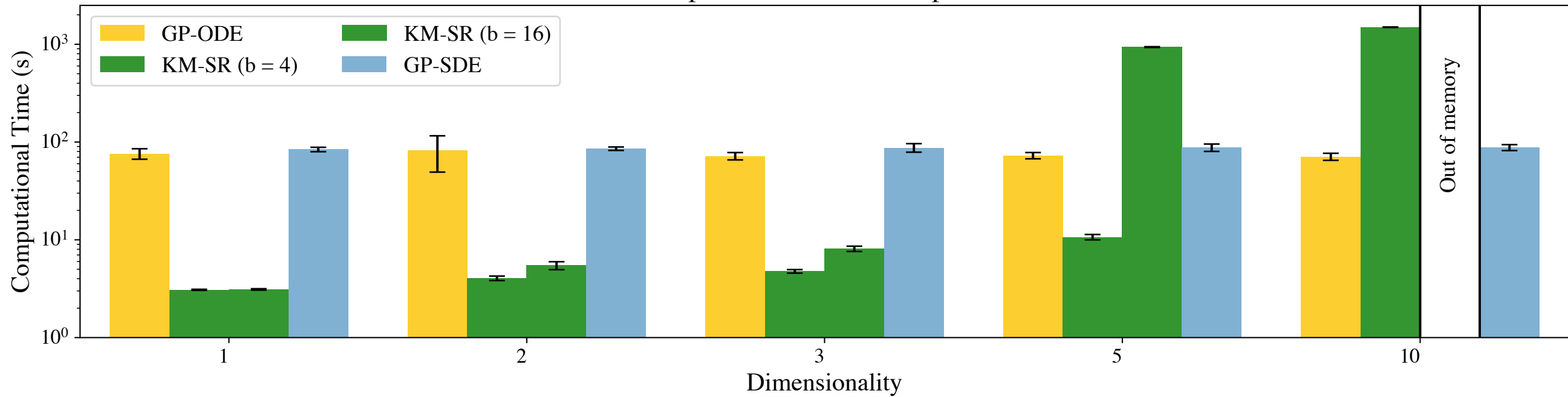
Computational Time Comparison
