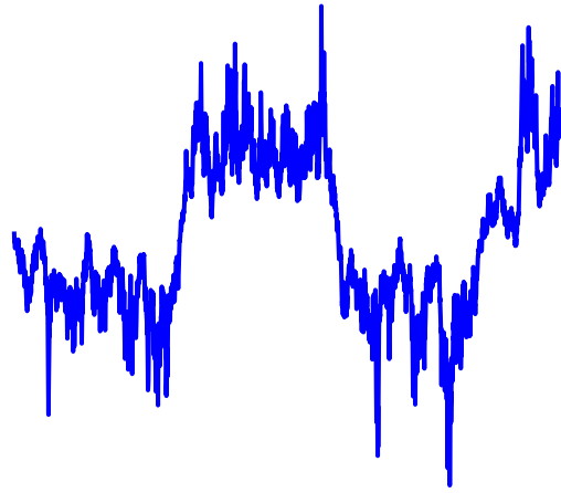
Double Well
