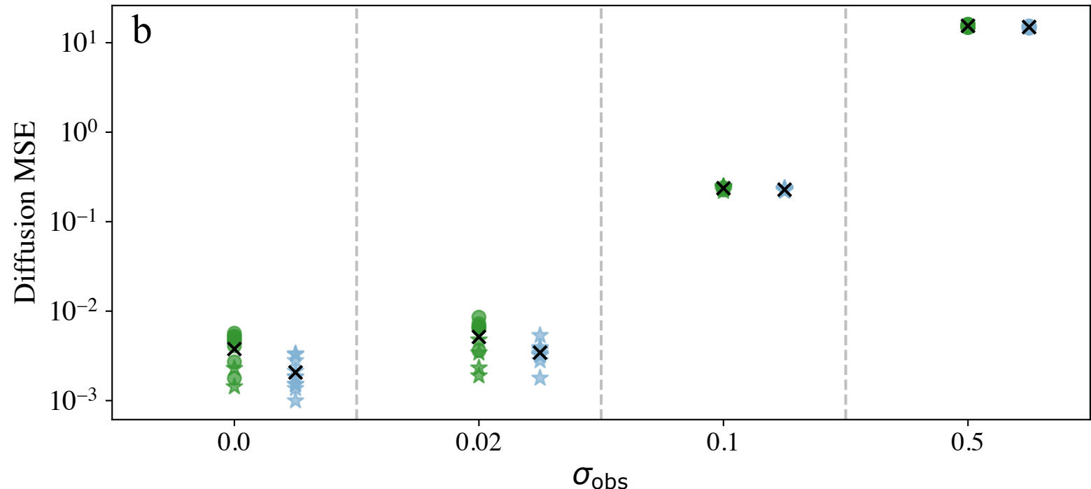
Double Well with observation noise
