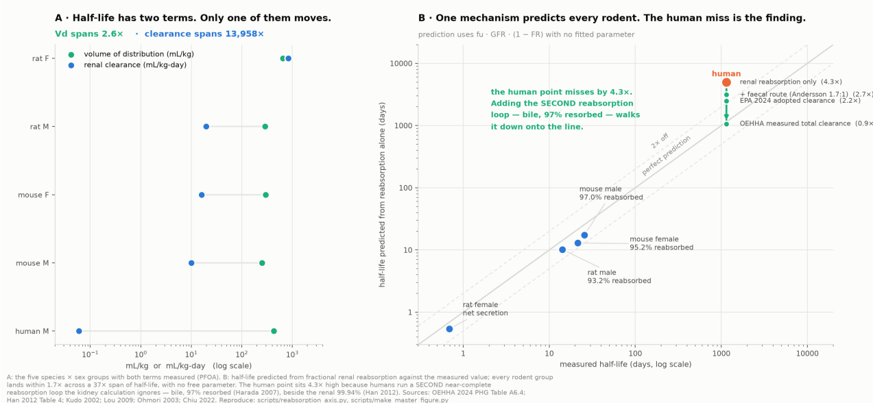
PFAS half-lives differ between species because of how much is reabsorbed, not how much is distributed
