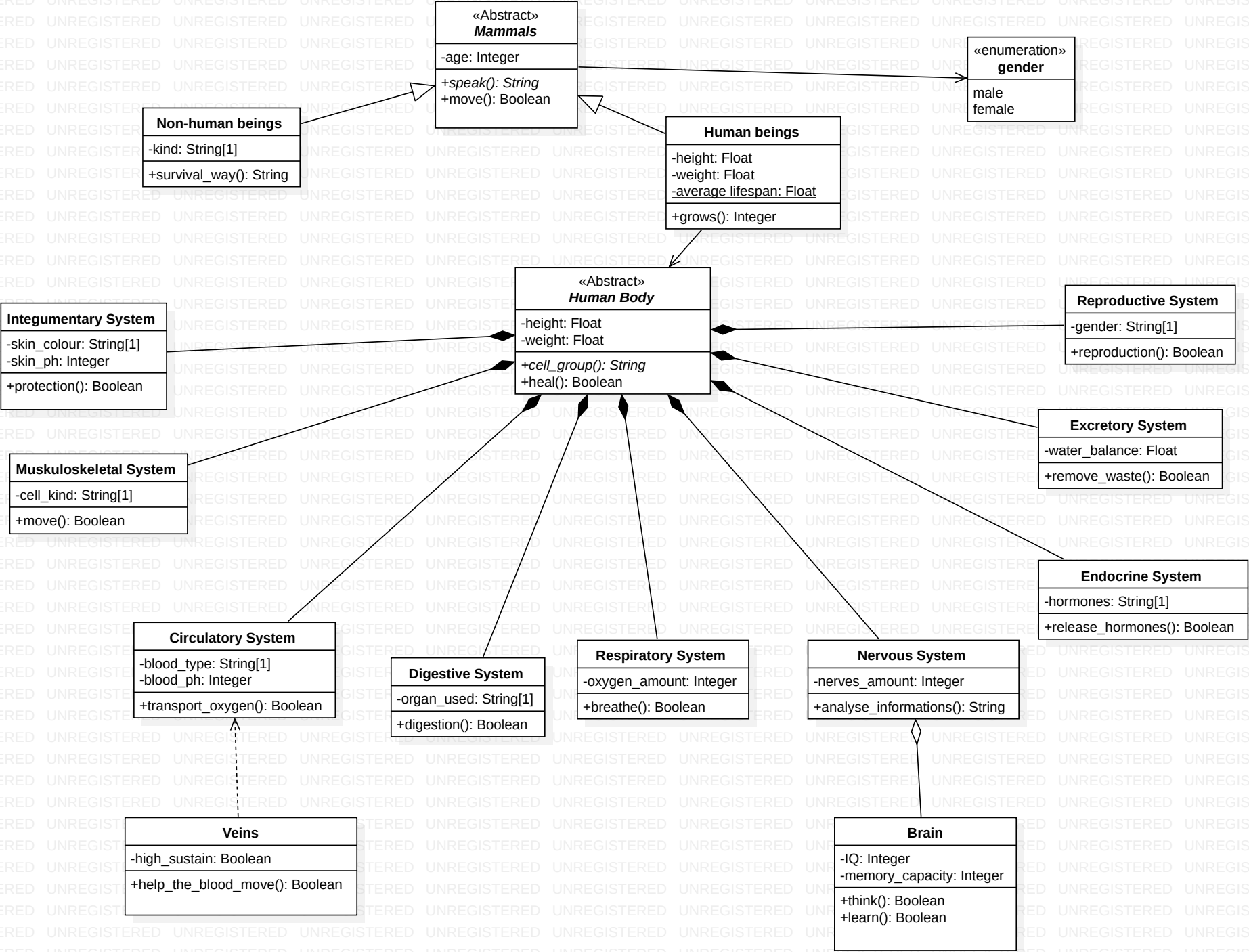
Model1::ClassDiagram1
