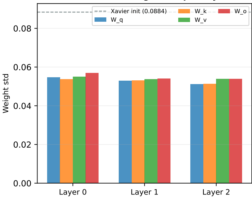
B. Attention weight std per layer
