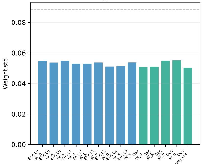
D. All attention weights: encoder vs decoder
