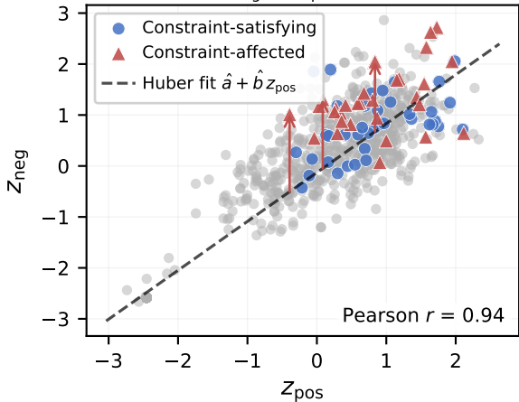
Raw: z_{\text{neg}} vs z_{\text{pos}} (qid 355)
