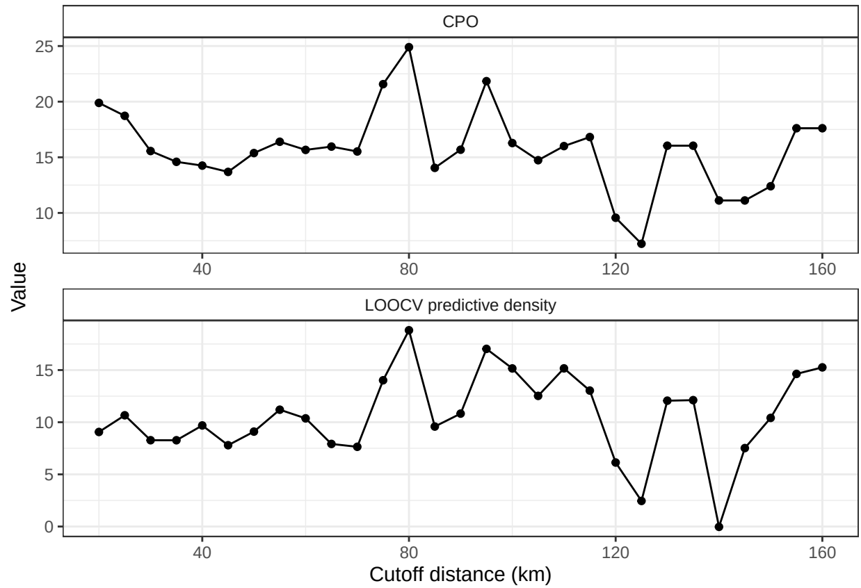
Figure 10: Predictive density calculated with Leave One Out Cross Validation (LOOCV) and the the conditional predictive ordinate, using sampled temperature from the June 2018 WCBTS survey. Estimates are shown for a subset of cutoff distances evaluated (x-axis).
