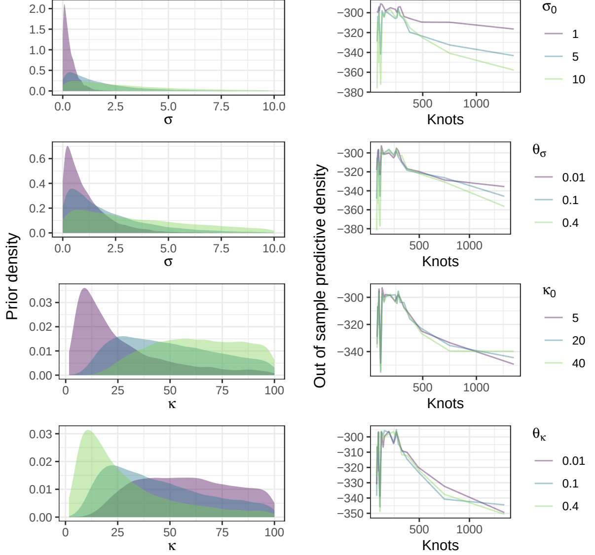
Figure 9: Prior sensitivity for Dover Sole presence-absence model, as a function of number of knots (using cutoff values from 3-120km) and hyperparameters of the Matern function.
