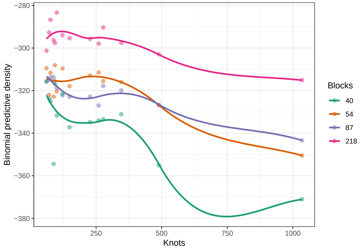
Figure 7: Binomial predictive density for Dover Sole, as a function of number of knots and number of spatial blocks used for 40-fold spatial cross-validation. Cutoff values between 5-135km are used across all scenarios.
