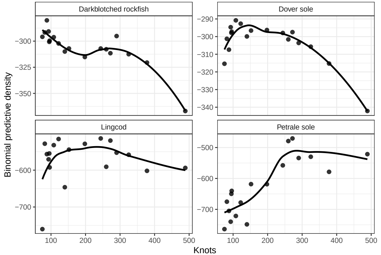
Figure 8: Binomial predictive densities for four species from the WCBTS survey, as a function of number of knots (using cutoff values from 3-120km). Estimation is done using Template Model Builder (TMB) instead of INLA.
