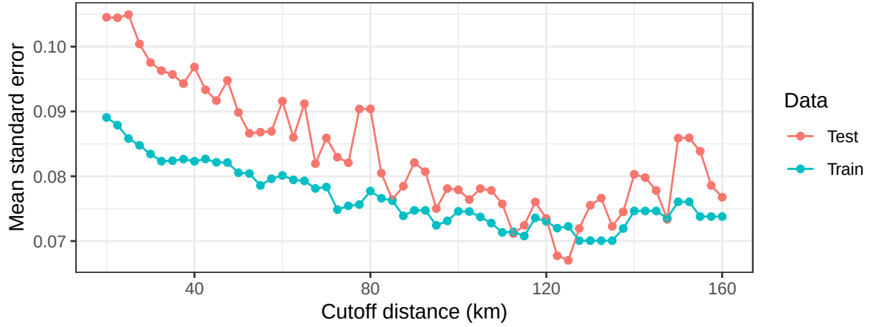
Figure 2: Mean standard errors of predictions for models of ocean temperature in the WCBTS survey, June 2018. Mean standard errors are calculated across all data points in the respective set ( n = 150 train, 25 test).
