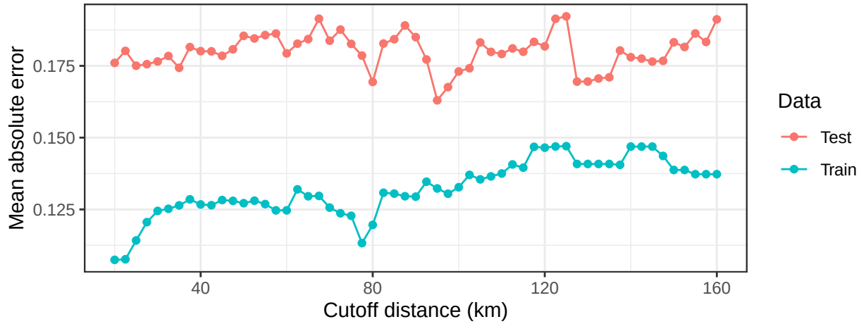
Figure 3: Mean absolute errors of predictions for models of ocean temperature in the WCBTS survey, June 2018. Mean absolute errors are calculated across all data points in the respective set ( n = 150 train, 25 test).
