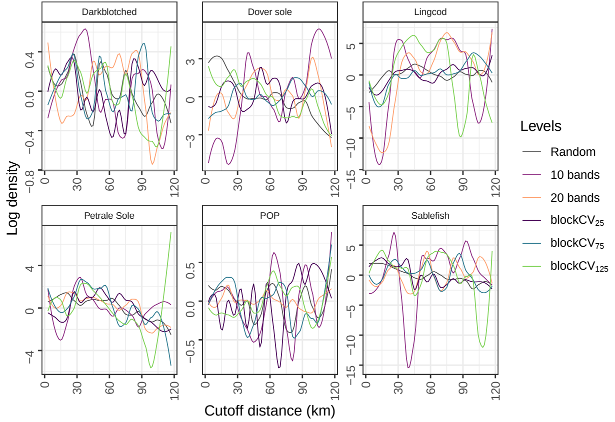
Figure 7: Binomial predictive densities for occurrence models for six species from the WCBTS survey, as a function of cutoff distances (larger cutoff distances correspond to coarser meshes).
