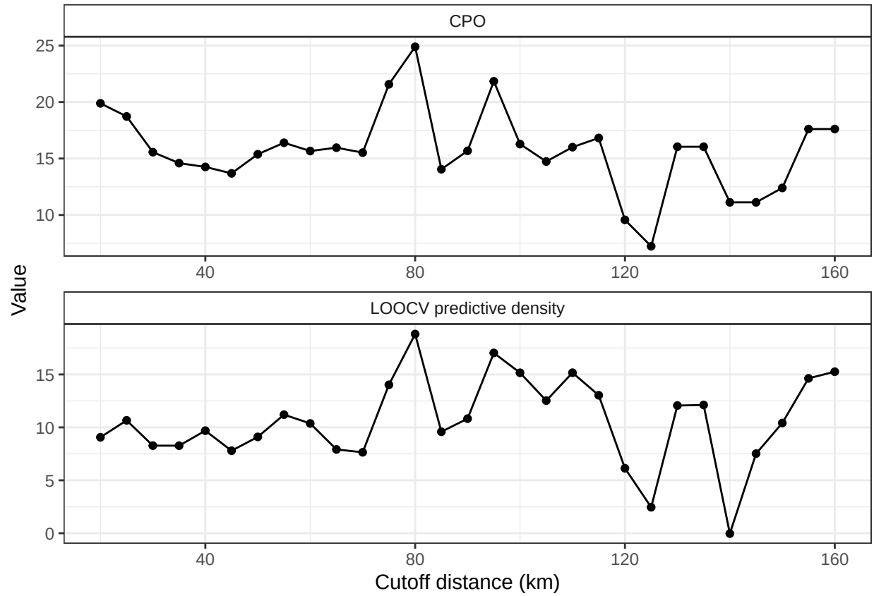
Figure 6: Predictive density calculated with Leave One Out Cross Validation (LOOCV) and the conditional predictive ordinate (CPO), using sampled temperature from the June 2018 WCBTS survey. Estimates are shown for a subset of cutoff distances evaluated (x-axis).
