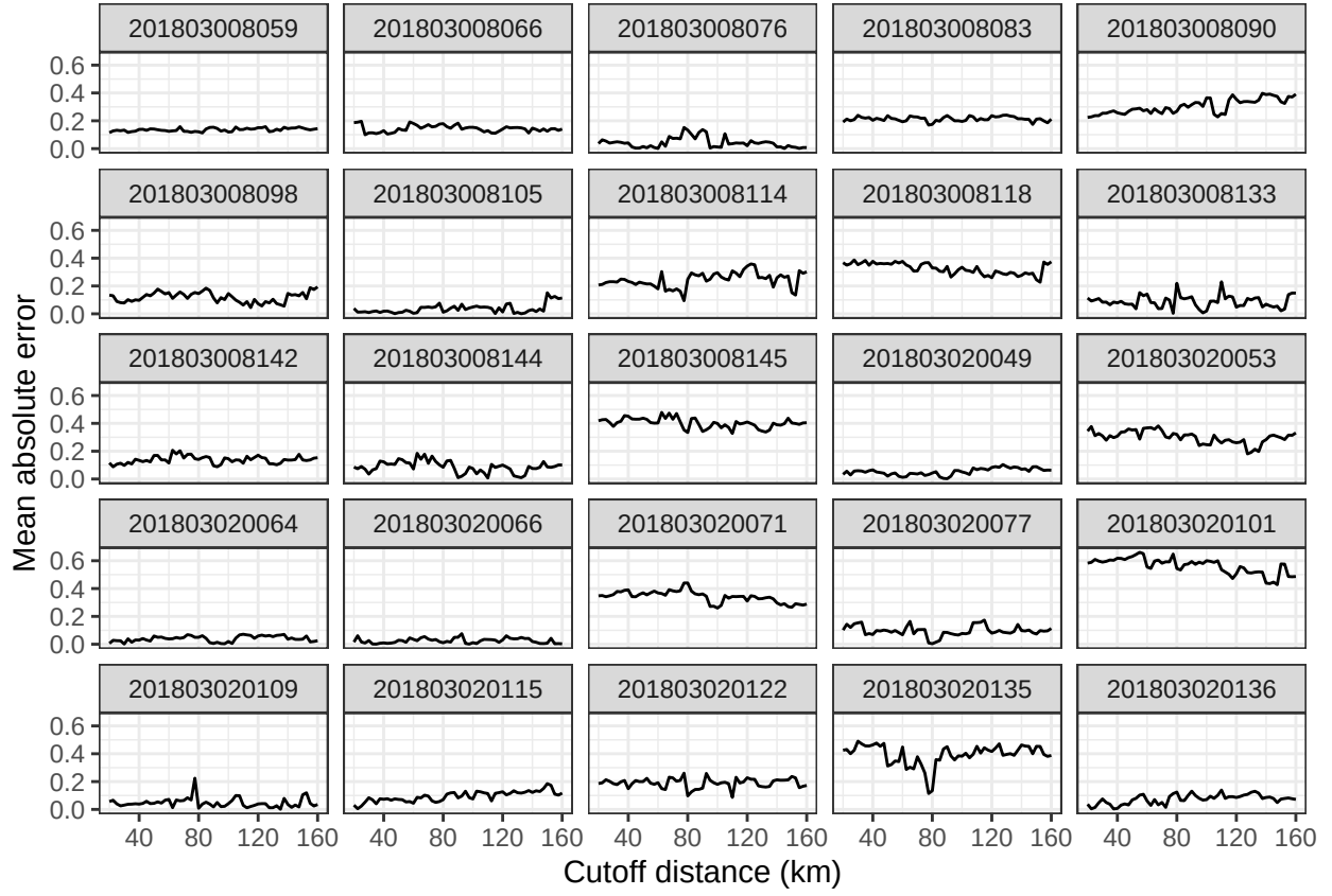
Figure 5: Mean absolute errors of predictions for models of ocean temperature in the WCBTS survey, June 2018. Estimates are shown for each held out trawl in the test set.
