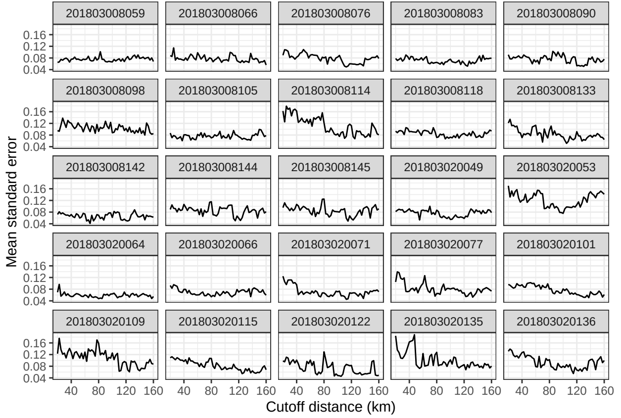
Figure 4: Mean standard errors of predictions for models of ocean temperature in the WCBTS survey, June 2018. Estimates are shown for each held out trawl in the test set.
