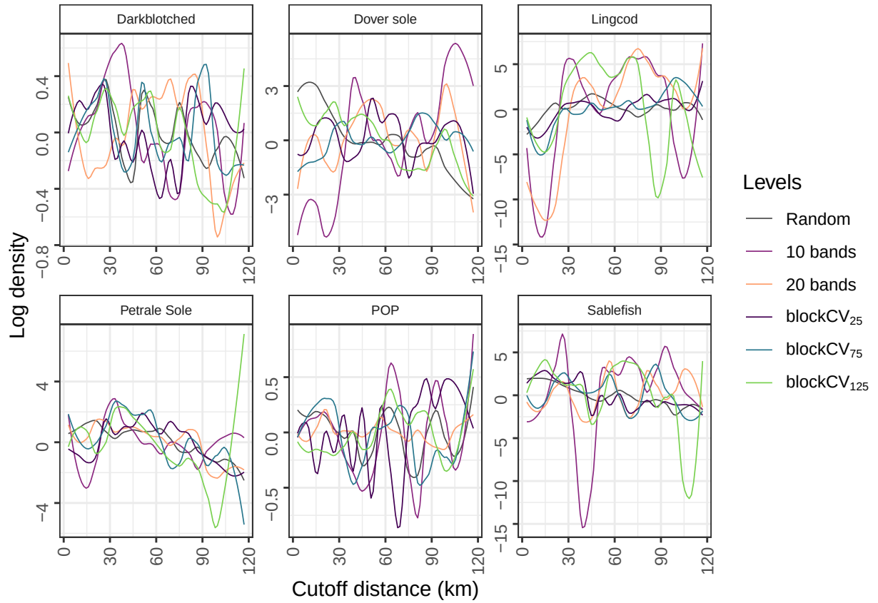
Figure 3: Binomial predictive densities for occurrence models for six species from the WCBTS survey, as a function of cutoff distances (larger cutoff distances correspond to coarser meshes). Range values of 25, 75, and 125 in the blockCV package translate to 218, 54, and 25 blocks. All series are centered to be on similar scales.
