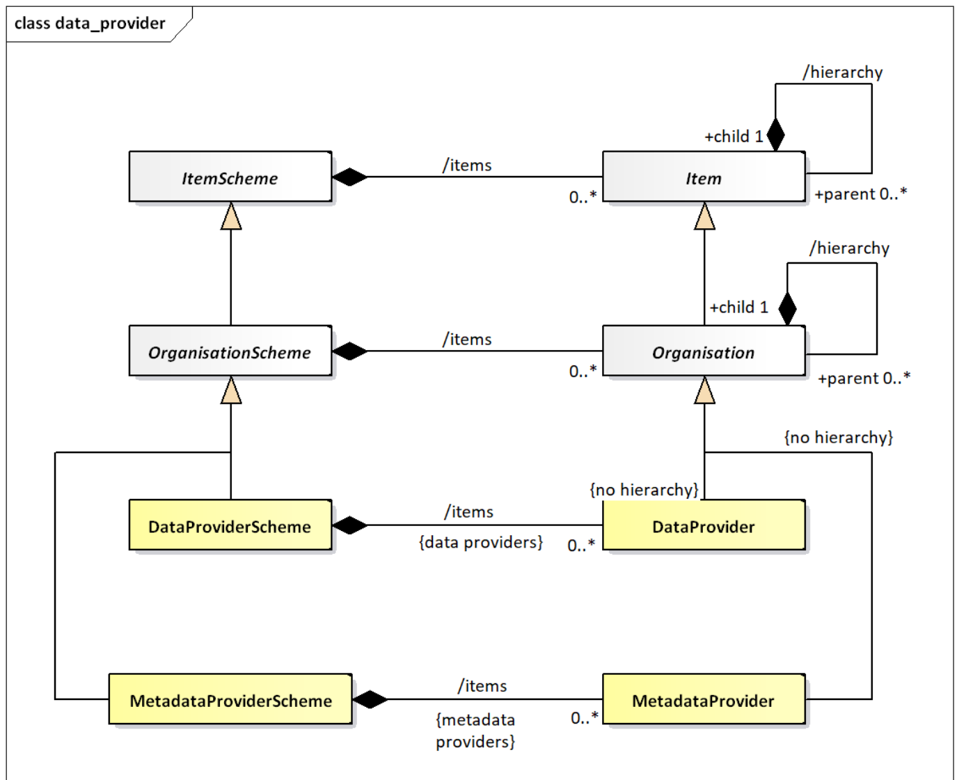
Figure 11. SDMX-IM of the Data Provider
