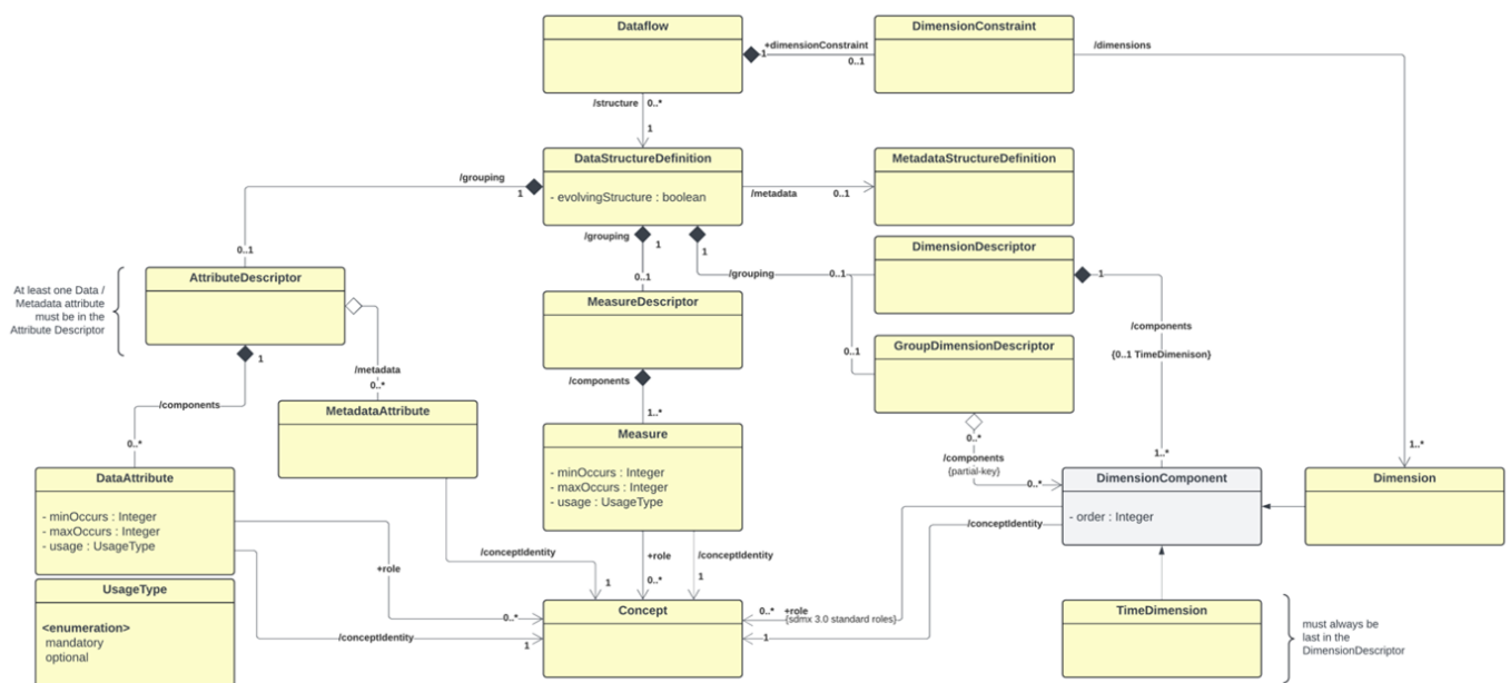
Figure 28. Relationship class diagram of the Data Structure Definition excluding representation
