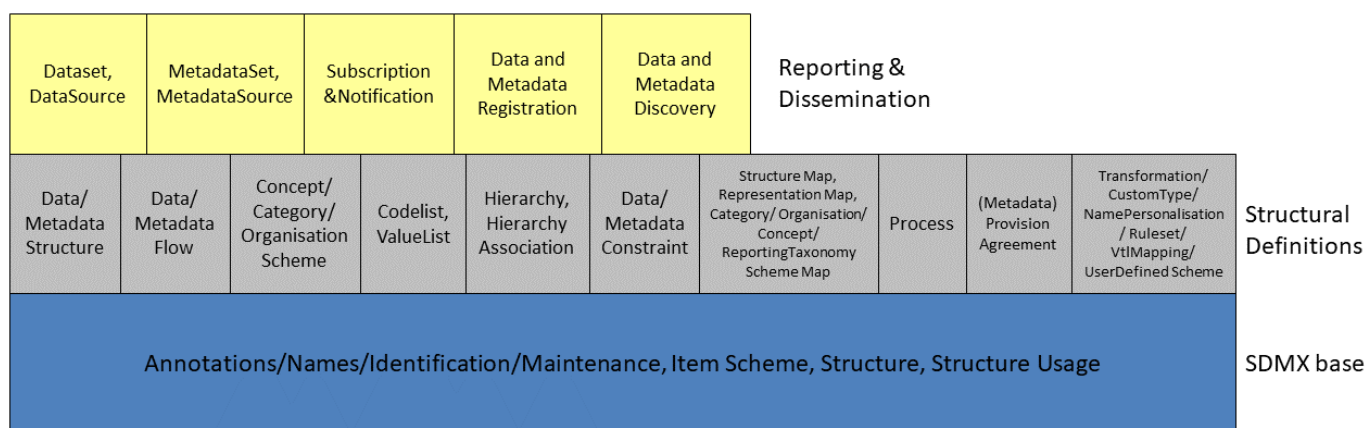
Figure 6. SDMX Information Model version 3.0 package structure
