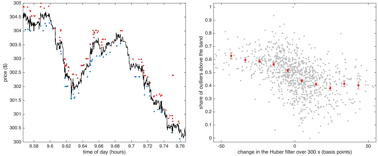
Figure 7: Outliers & robust price for CRWD on 16 October 2024. Left: the 12 minutes with the largest move in the Huber filter that day; outliers above Y_t - \theta_t > \delta_{t-1} in red, outliers below Y_t - \theta_t < -\delta_{t-1} in blue, Huber filter in black. Right: over the 12 trading days, the 300 second empirical conditional probability that outliers are above (rather than below) the Huber band against the 300 second change in the Huber filter in basis points: light points are single bins, the line & bars are means & s.e.
