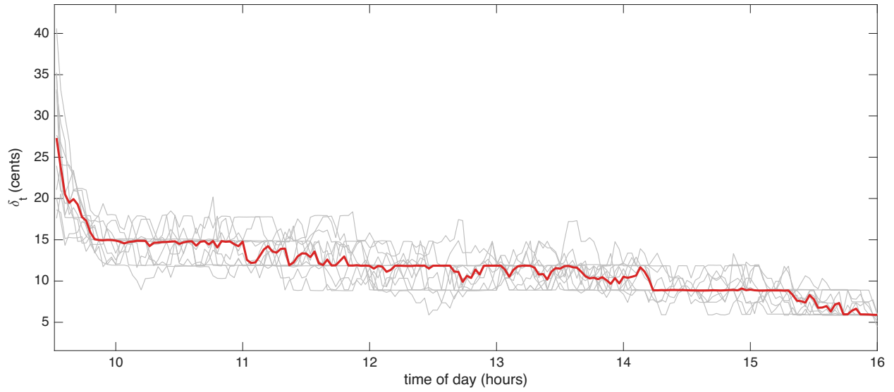
Figure 3: Huber threshold \delta_t in cents through the trading day, for 12 CRWD trading days in Oct 2024 (grey lines) and their median (red line).
