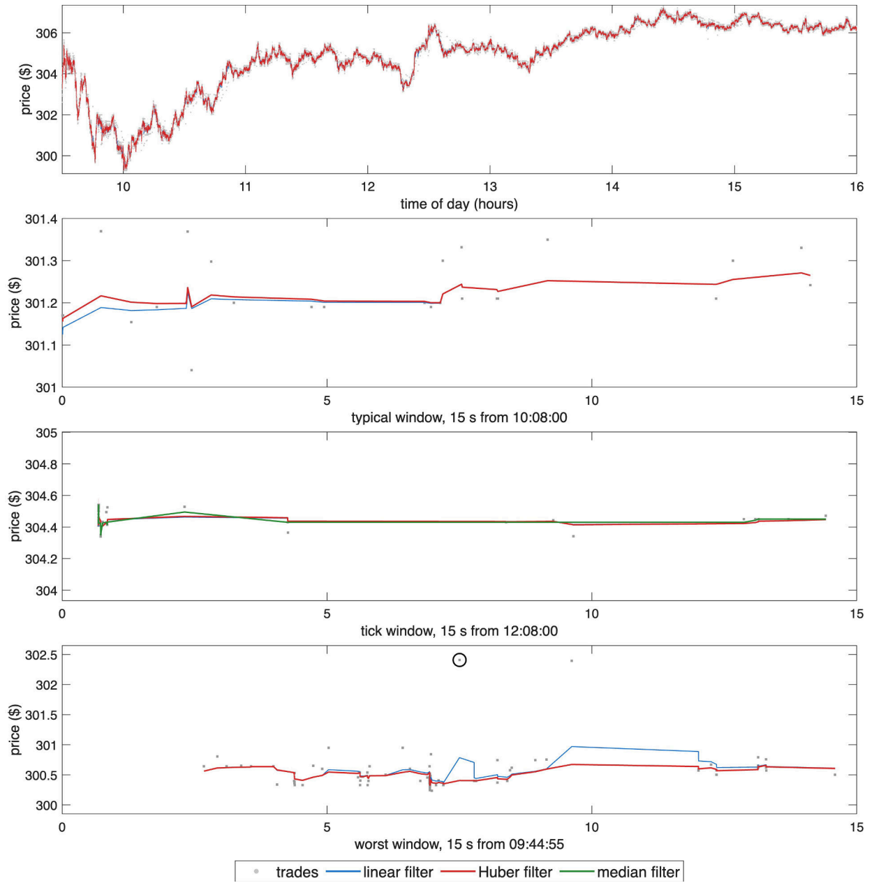
Figure 1: CRWD trades (grey points), the linear filter and the Huber filter, 16 October 2024. Top: full trading day. 2nd: 15-second window at the day's median trade count, from 10:08:00. 3rd: 15-second window at 12:08:00 in which the price reverses direction most often, with the median filter m_t added. Bottom: 15-second window around the largest Huber residual after 09:45, circled.
