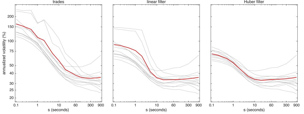
Figure 4: Volatility signature curves for CRWD over the 12 trading days in Oct 2024. The annualized vol \hat{\sigma}100\sqrt{252} from the returns \hat{X}_t - \hat{X}_{t,s} of Table 2, against the lag s in seconds, both axes on log scales, for: raw trades, linear filter & Huber filter. Grey lines are the individual trading days & the red line is the square root of the 12 day average of their squares. The linear & Huber returns carry the finite-sample correction c_{t,s} of the paper; the raw trades are unaffected by it.
