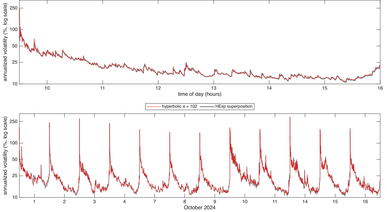
Figure 6: Hyperbolic against superposition weights for CRWD over 12 trading days in Oct 2024, the diurnally adjusted \hat{\sigma}(u)100\sqrt{252} at s = 1 second from the Huber filter, shown as annualized vol in % on a log10 scale. The only difference between the 2 paths is the weight function: the hyperbolic weights with a = 102 in red, drawn on top, and the HExp superposition in grey, 4 exponential components with half lives of 60, 600, 3600, 23400 seconds. Hyperparameters minimize the QLIKE objective. Top: 16 October 2024, bottom: 12 days.
