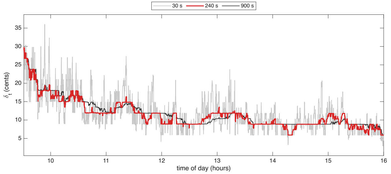
Figure 2: The Huber threshold \delta_t in cents for CRWD on 16 October 2024, with half-lives of 30, 240, 900 seconds. The 240-second half-life, in red, is used.
