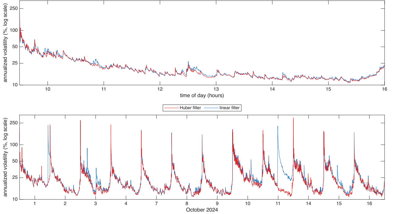
Figure 5: Filtered spot volatility for CRWD over 12 trading days in Oct 2024, the diurnally adjusted estimator \hat{\sigma}(u)100\sqrt{252} at s = 1 second with hyperbolic weights, Mandelbrot parameter a = 102 , with the input prices computed using the Huber & linear filters, shown as annualized volatility in percent on a log10 scale. Top: 16 October 2024, bottom: 12 days.
