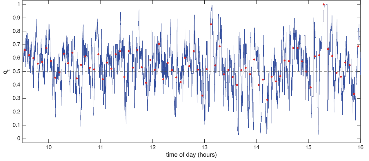
Figure 8: The directional conditional probability for CRWD, 16 October 2024. The filtered conditional probability q_t that an outlier lies above the robust Huber band, under exponential weights decaying in clock time with half life of 37 seconds; where fewer than two outliers remain in the weights it is drawn in grey. The dashed line marks 0.5. The red points are the empirical conditional probability using the 300 second bins of the previous figure.
