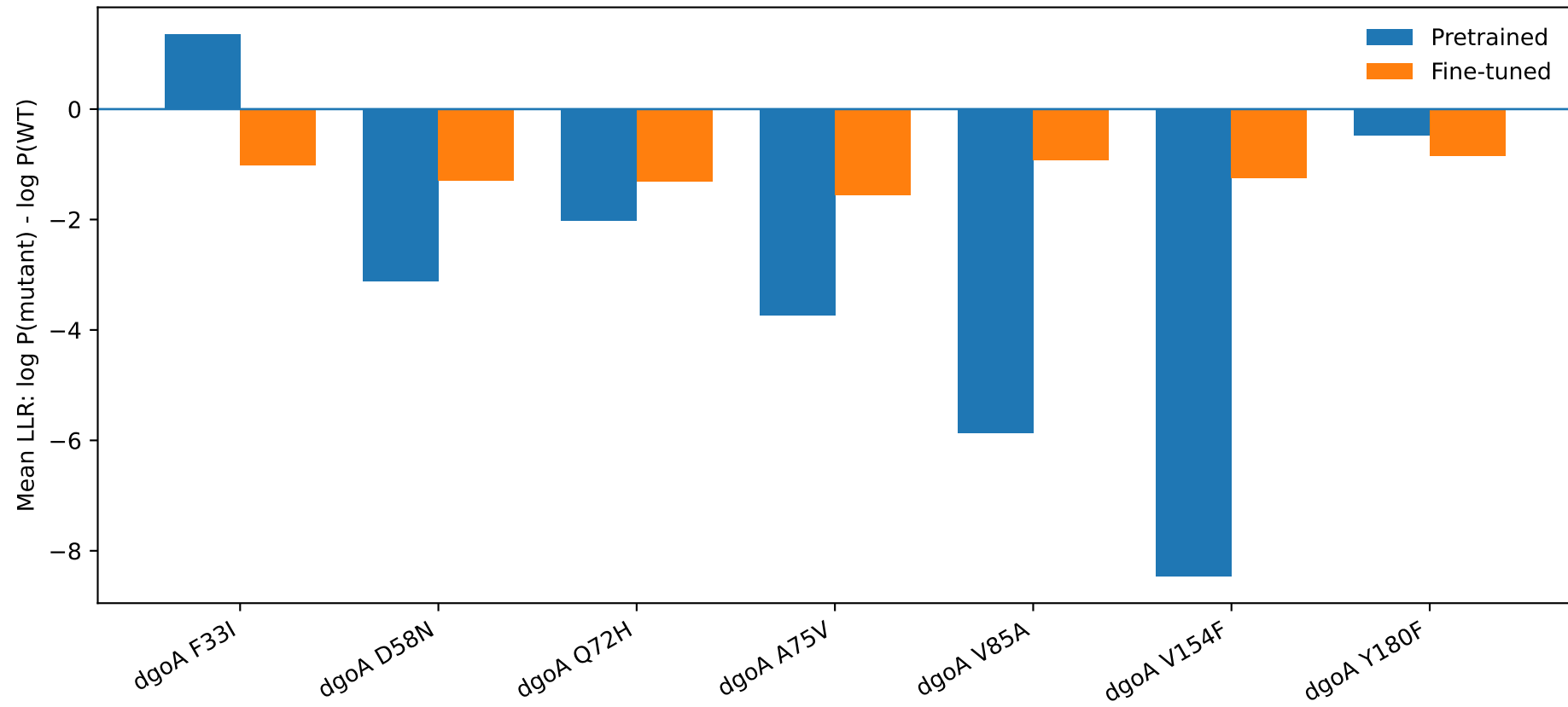
ESM-2 DgoA: pretrained vs fine-tuned ALE-site preference
