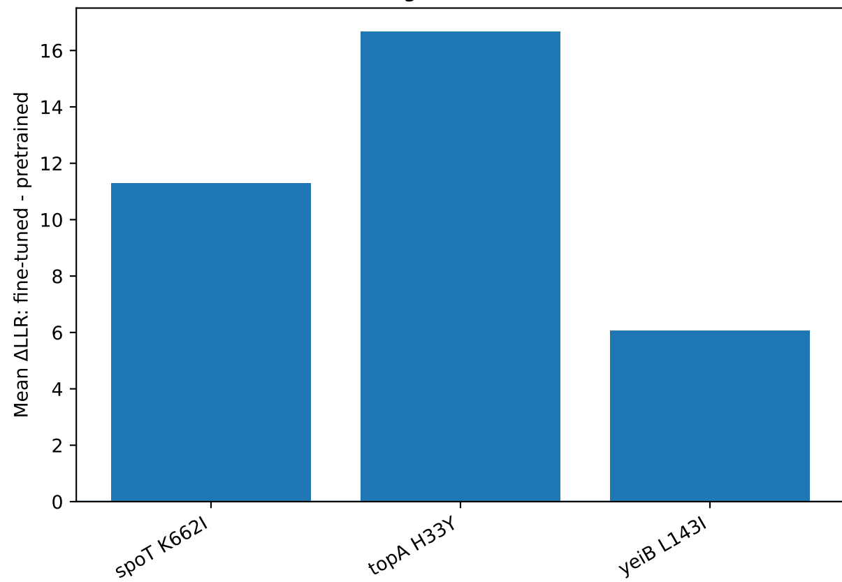
ESM-2 E. coli: fine-tuning shift toward ALE mutant residue
