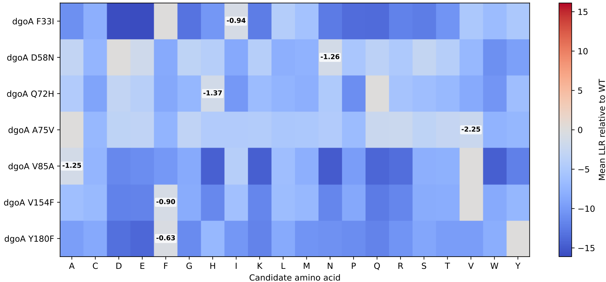
Fine-tuned mean amino-acid LLR at ALE sites
