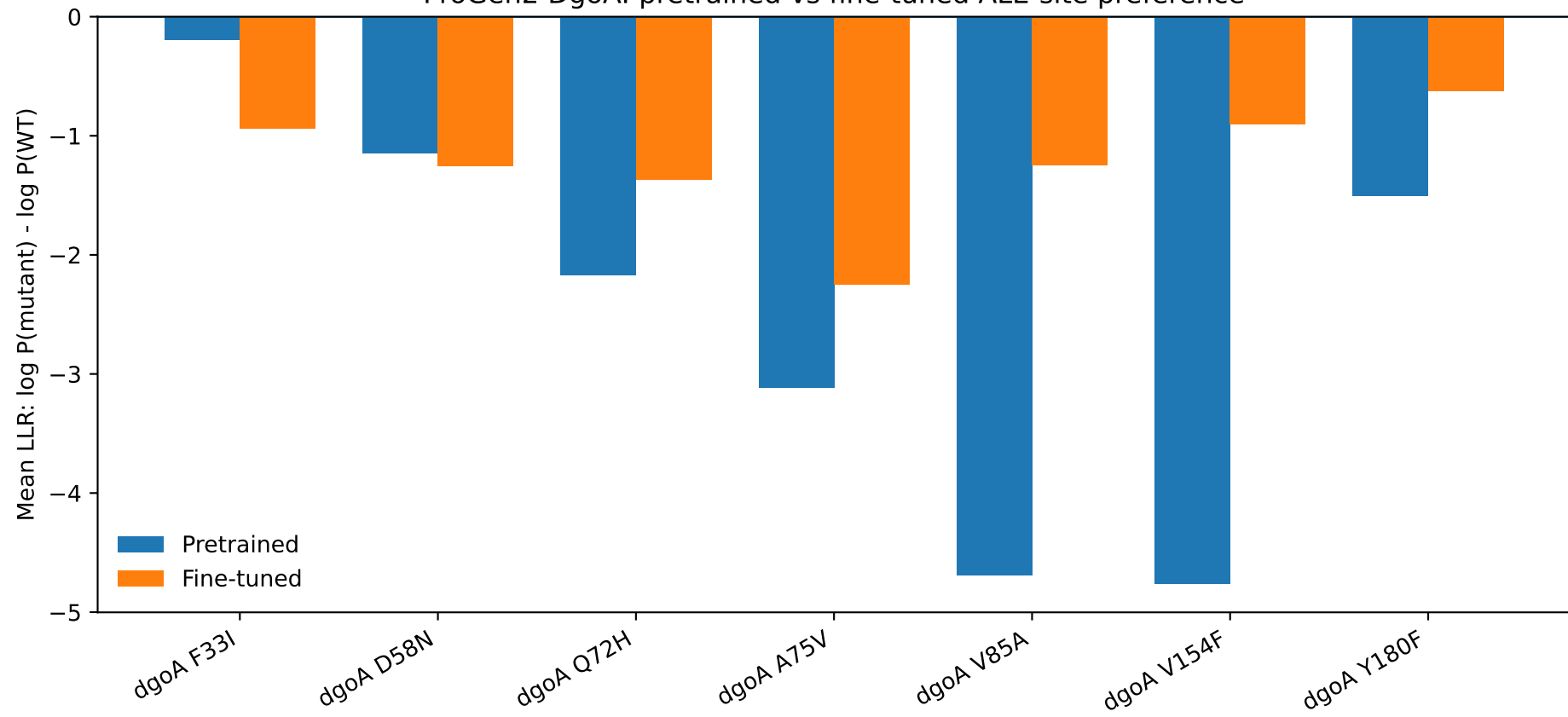
ProGen2 DgoA: pretrained vs fine-tuned ALE-site preference
