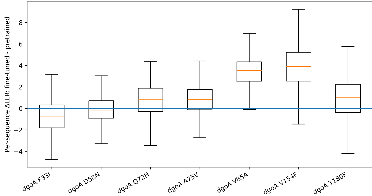
ProGen2 DgoA: per-sequence shifts across held-out homologs
