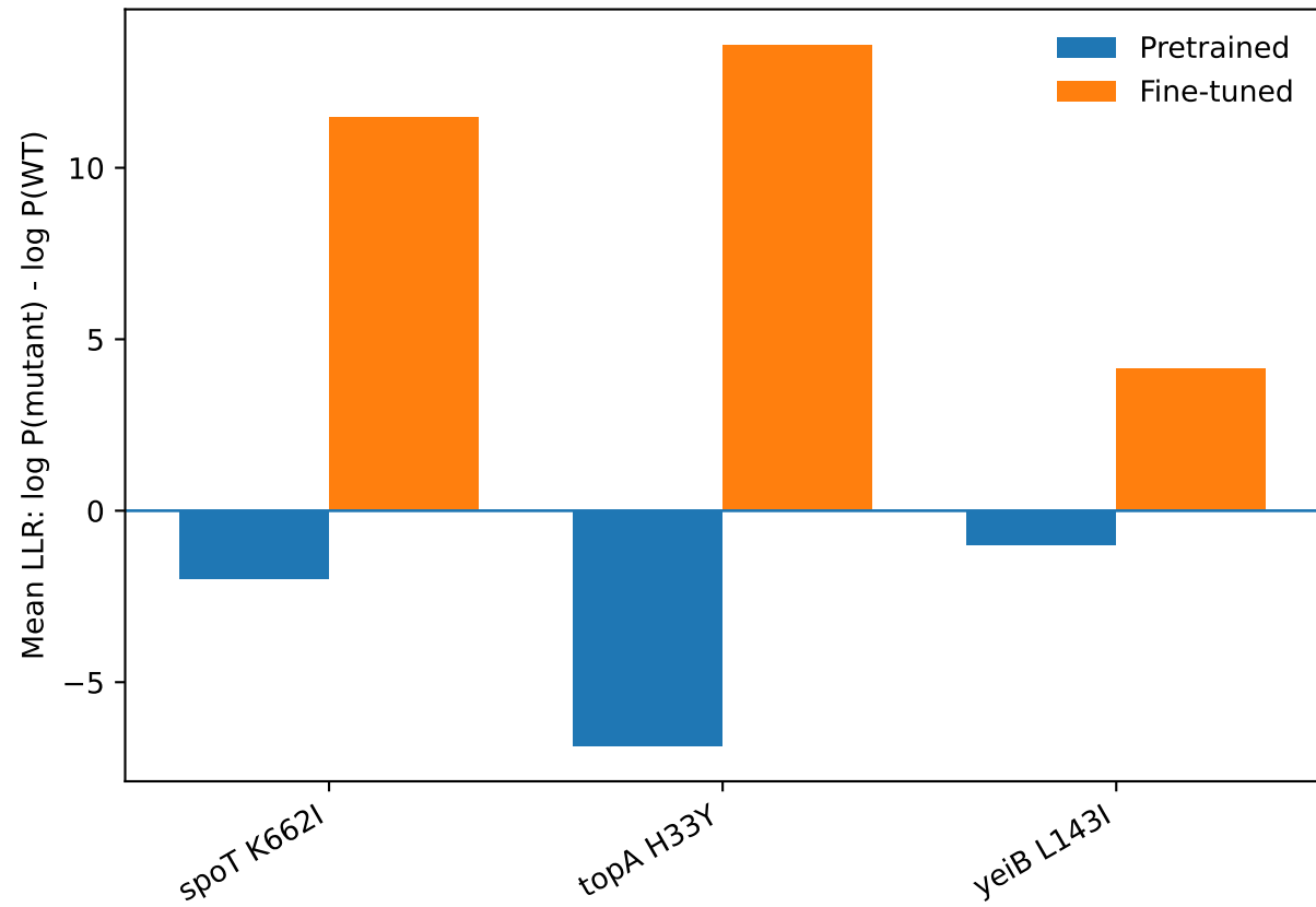
ProGen2 E. coli: pretrained vs fine-tuned ALE-site preference
