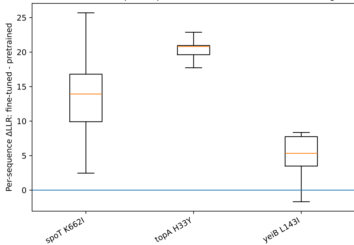
ProGen2 E. coli: per-sequence shifts across held-out homologs
