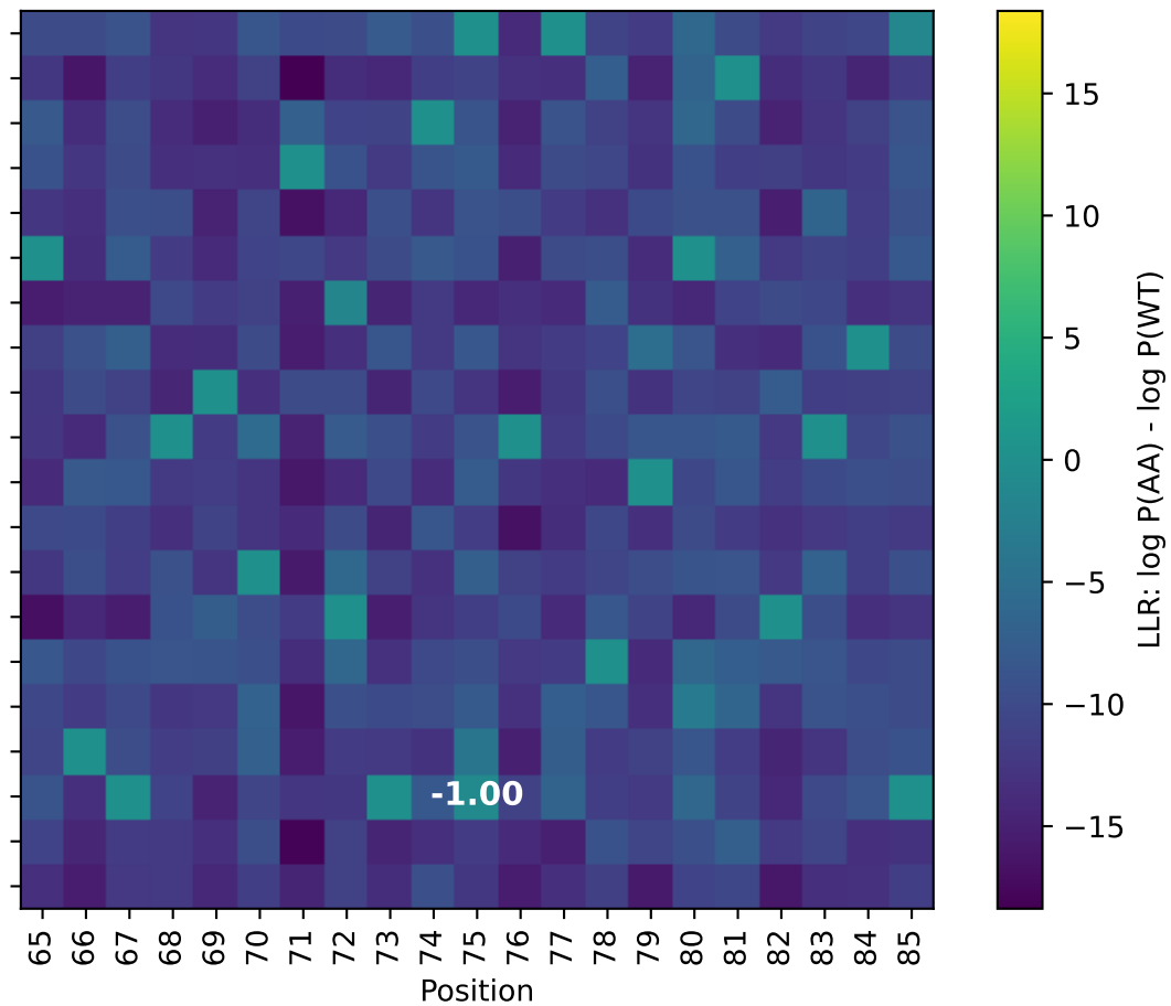
ESM-2 fine-tuned
