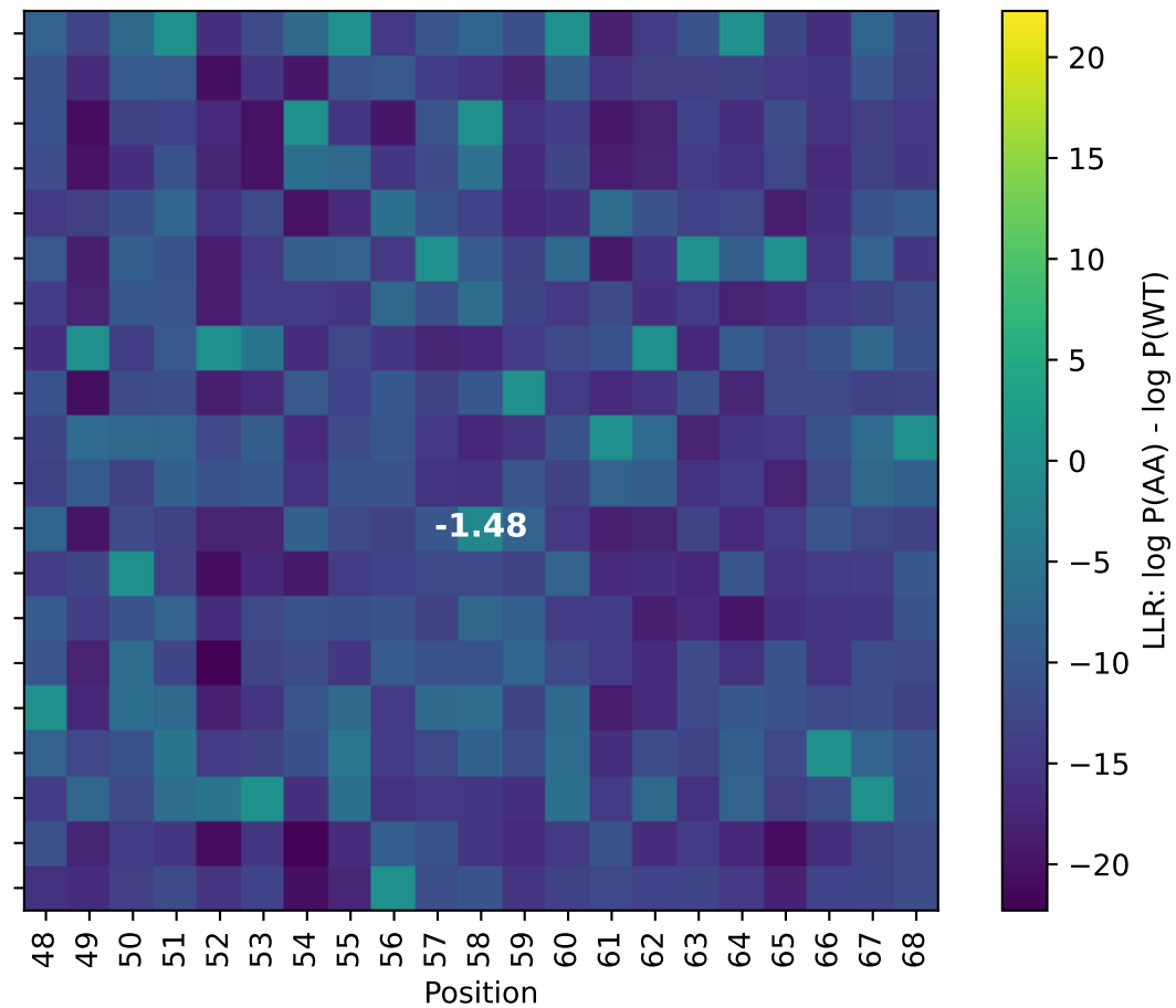
ProGen2 fine-tuned
