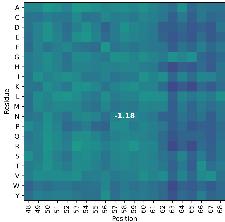
ProGen2 pretrained
