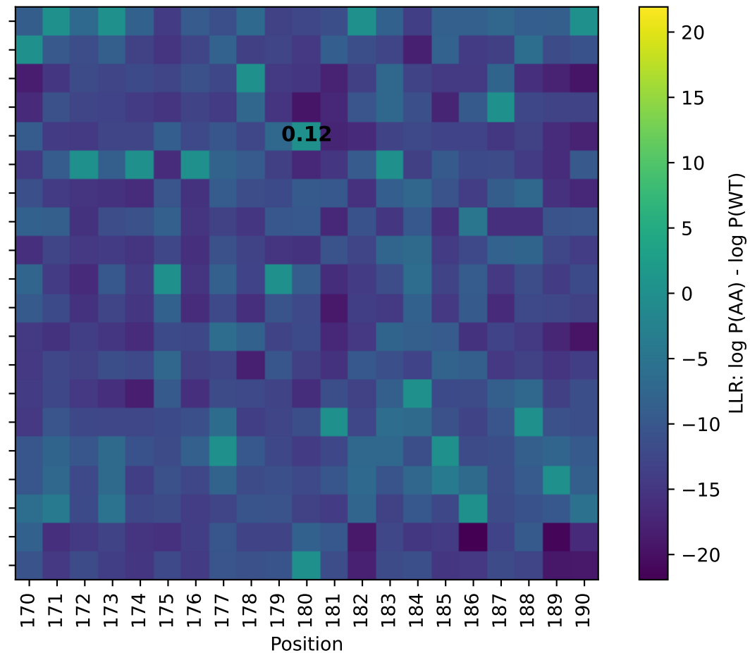
ProGen2 fine-tuned
