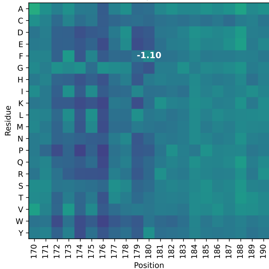
ProGen2 pretrained
