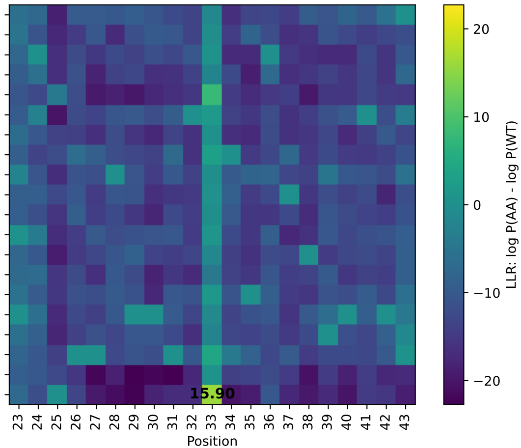
ProGen2 fine-tuned
