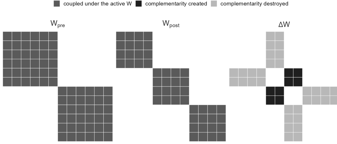
Figure 16: The K_{CC} switch. Left, the pre-shock interaction matrix W_{pre} ; centre, the post-shock W_{post} ; right, their difference. The shock schedule flips the weights of two XWX covariates at the midpoint, so actors carry their positions across a change in which components complement which.
