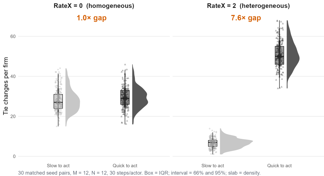
Figure 17: Rate separation. With RateX active, quick-to-act actors make 51.0 tie changes against 6.7 for slow-to-act (ratio 7.6) while the control arm sits at 1.05, with evaluation functions held identical across arms.
