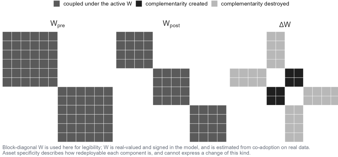
Figure 16: The K_{CC} switch. Left, the pre-shock influence matrix W_{\text{pre}} ; centre, the post-shock W_{\text{post}} ; right, their difference. The shock schedule flips the weights of two XWX covariates at the midpoint, so actors carry their positions across a change in which components complement which.
