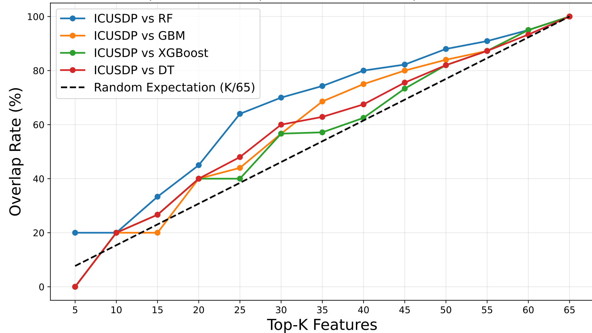
Top-K Feature Overlap between ICUSDP and Supervised Models
