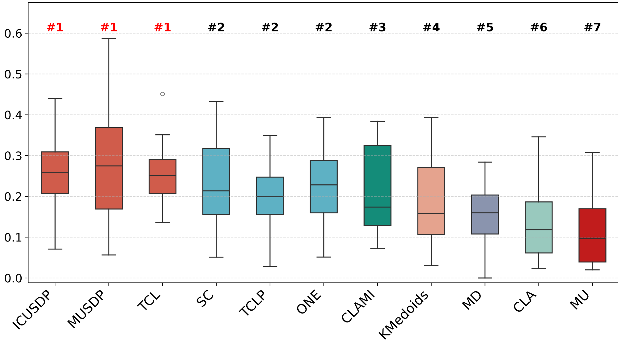
F-measure@20%LOC
