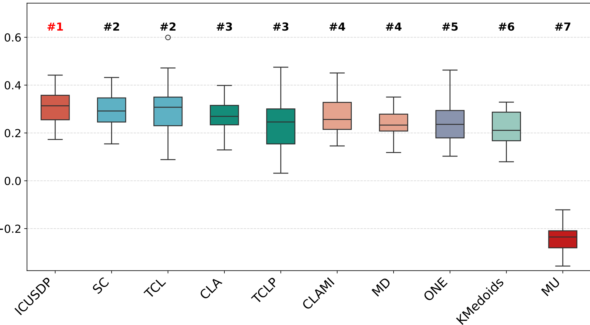
Comparison of Matthews Correlation Coefficient (MCC) in Unsupervised Methods
