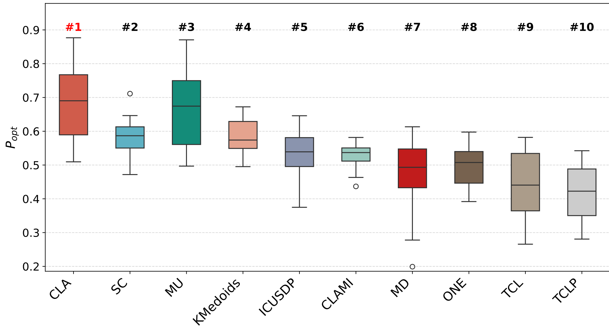
Comparison of P_{opt} in Unsupervised Methods
