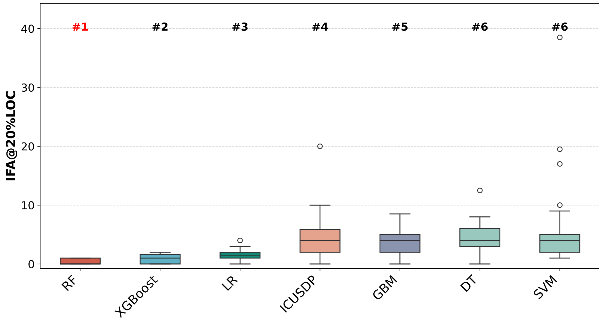
Comparison of IFA@20%LOC in Supervised Methods
