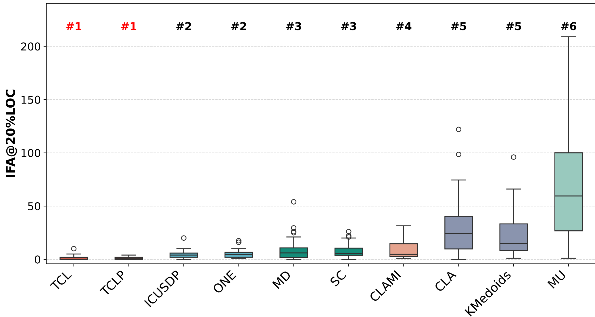
Comparison of IFA@20%LOC in Unsupervised Methods
