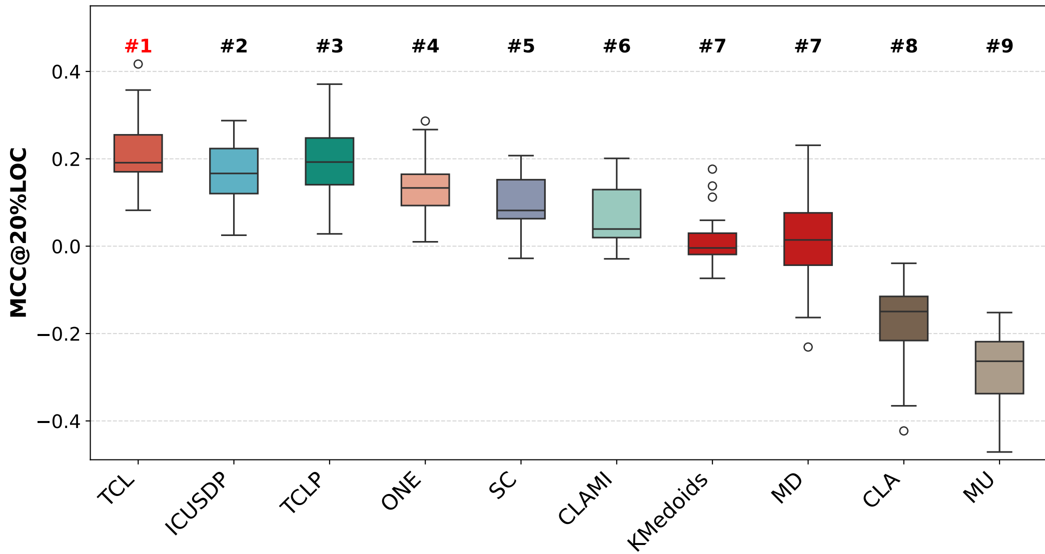
Comparison of MCC@20%LOC in Unsupervised Methods
