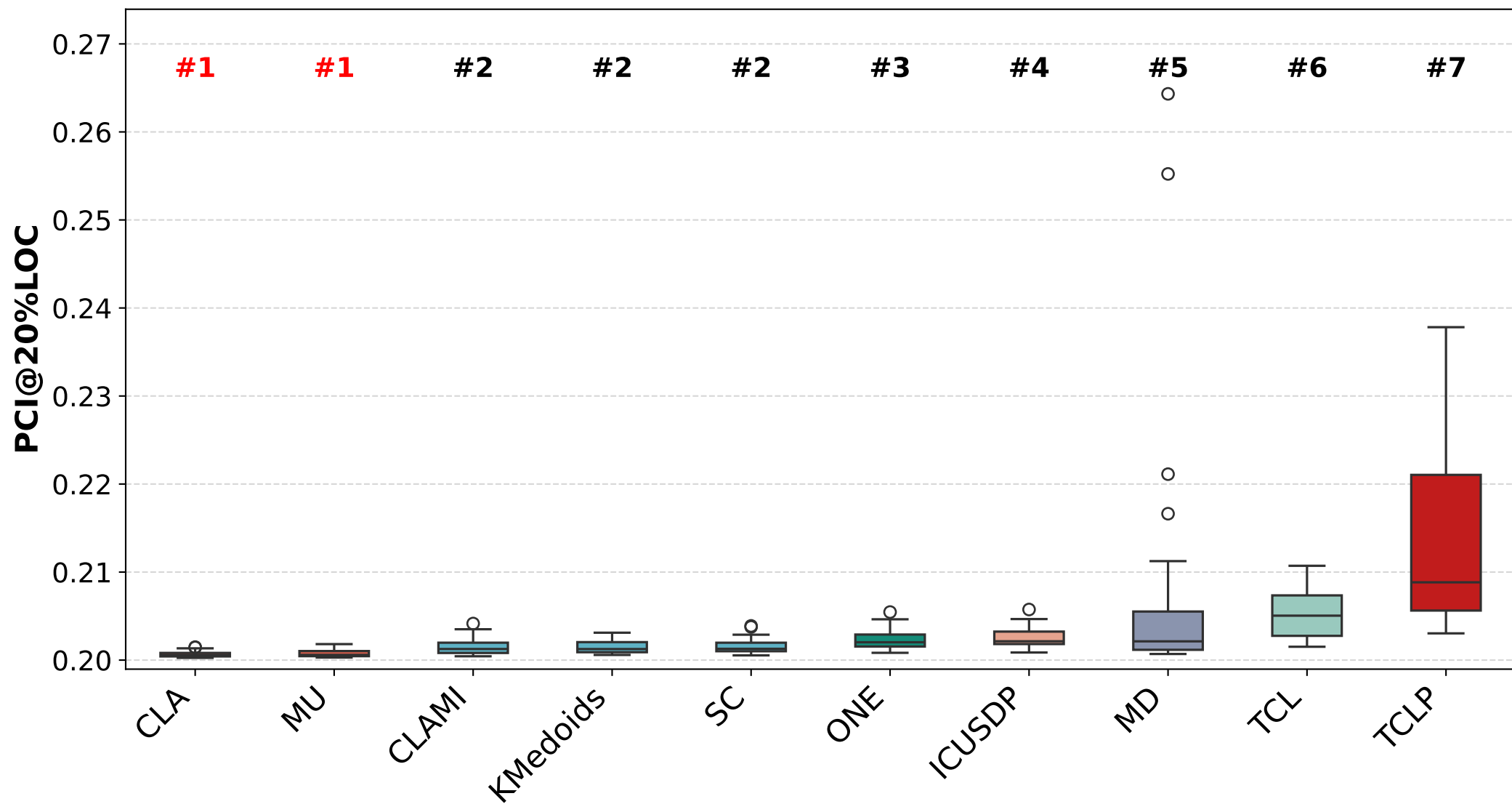
Comparison of PCI@20%LOC in Unsupervised Methods
