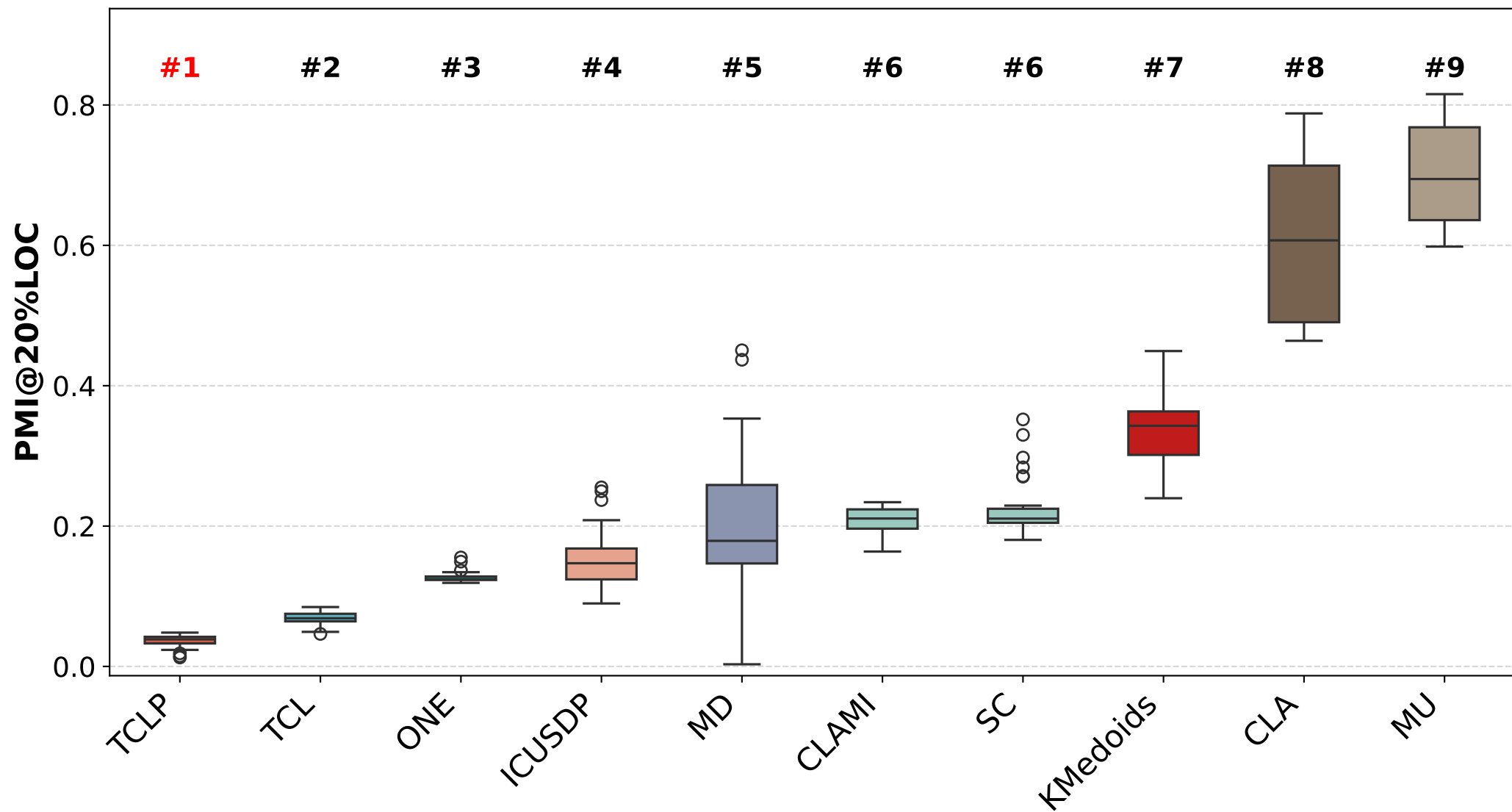
Comparison of PMI@20%LOC in Unsupervised Methods
