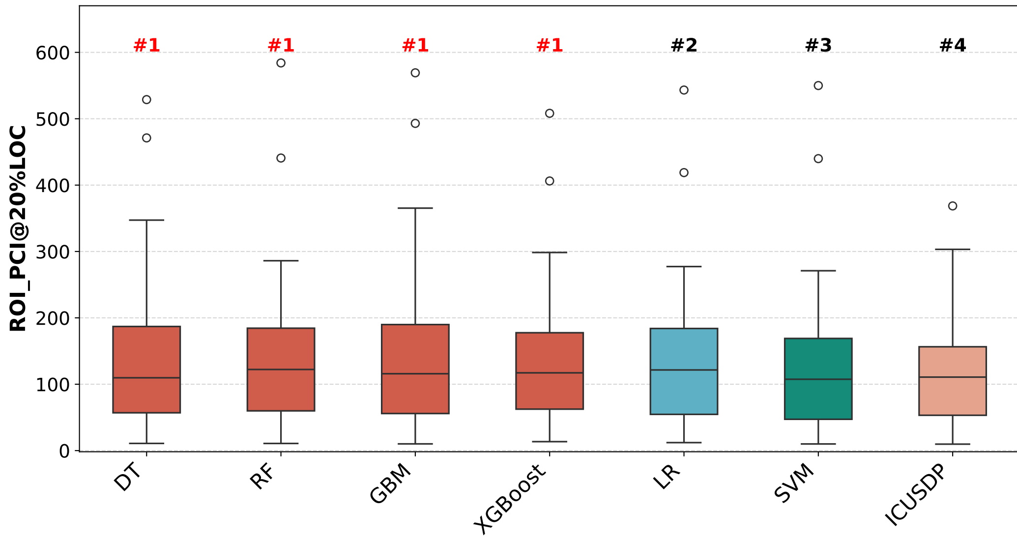
Comparison of ROI_PCI@20%LOC in Supervised Methods
