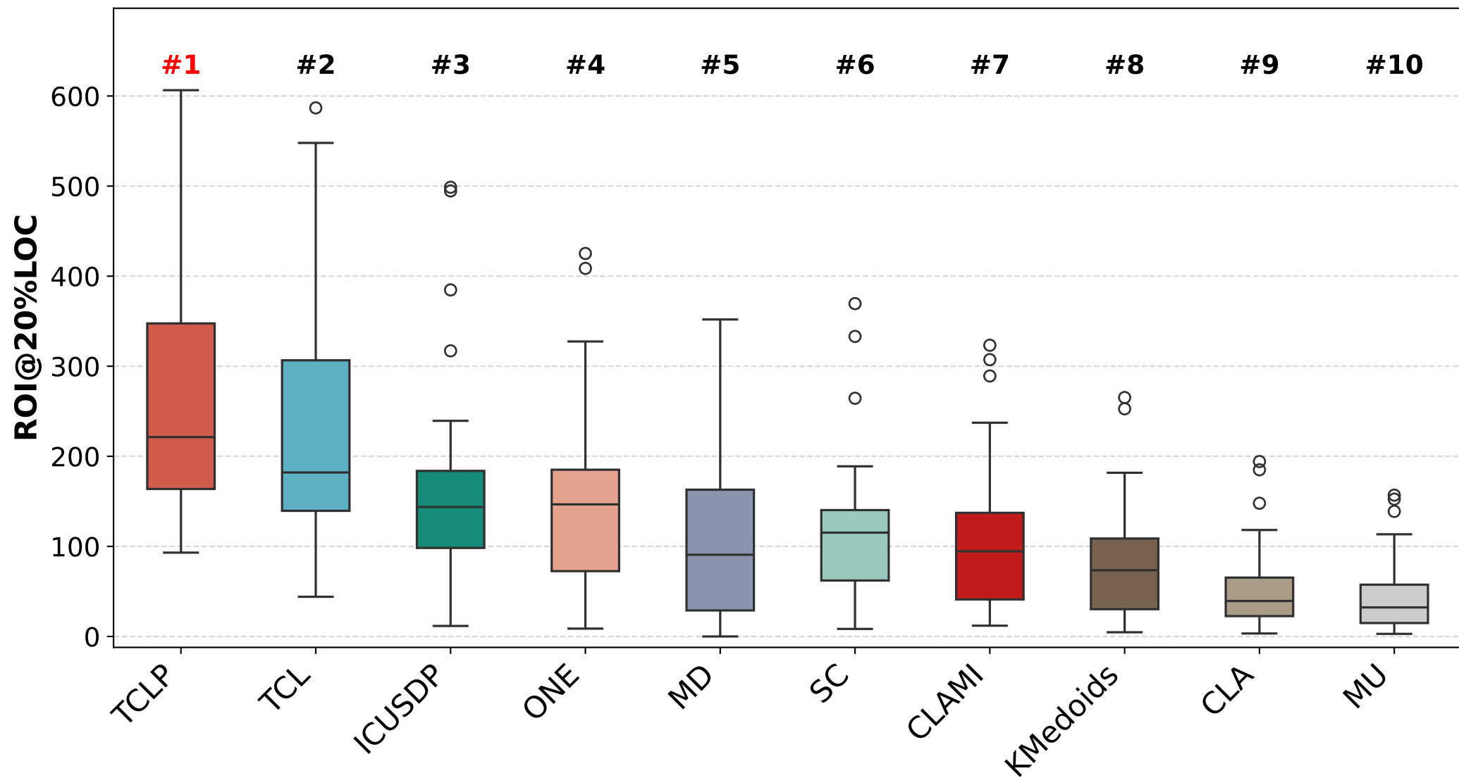
Comparison of ROI@20%LOC in Unsupervised Methods
