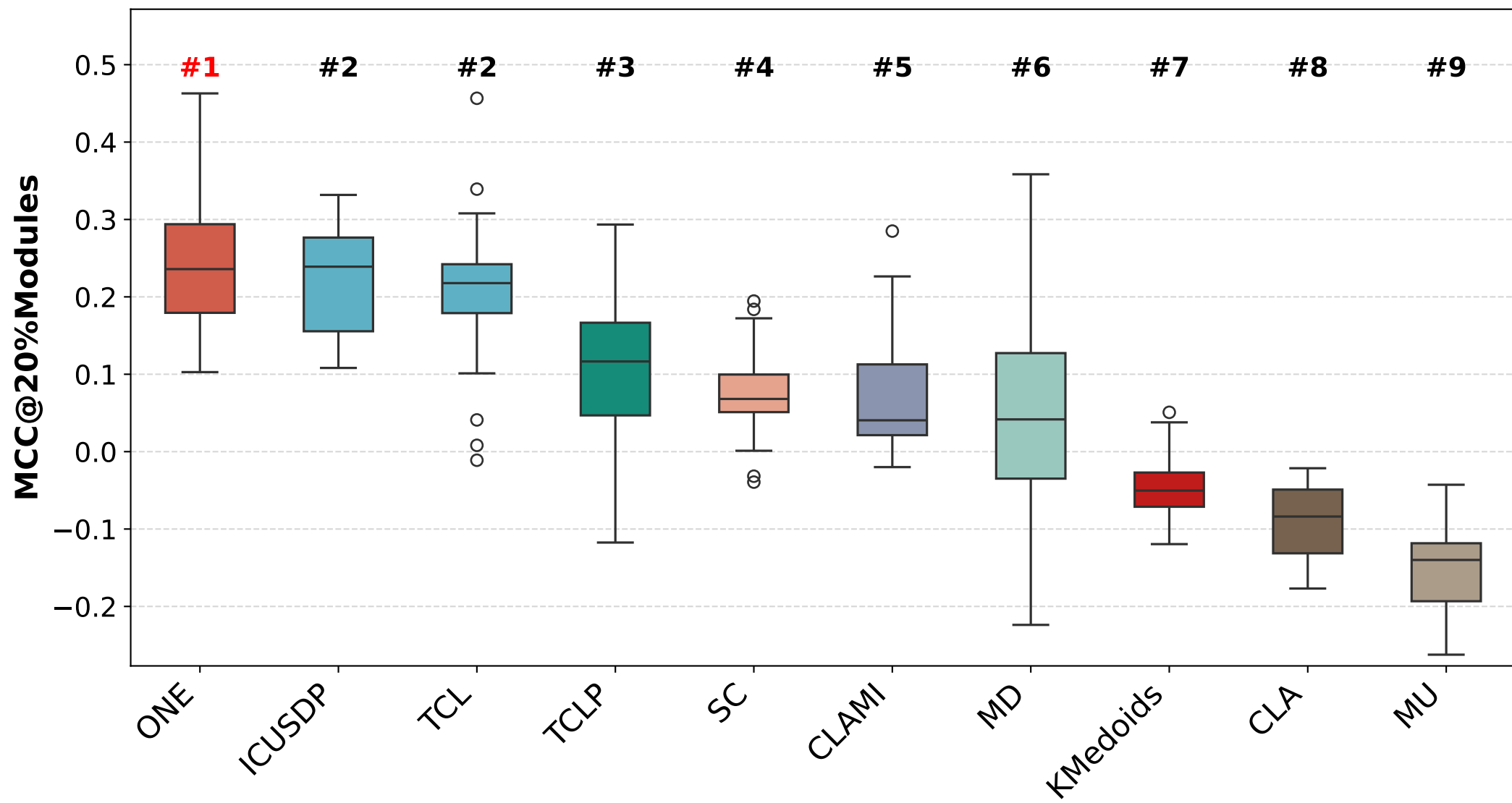
Comparison of MCC@20%Modules in Unsupervised Methods
