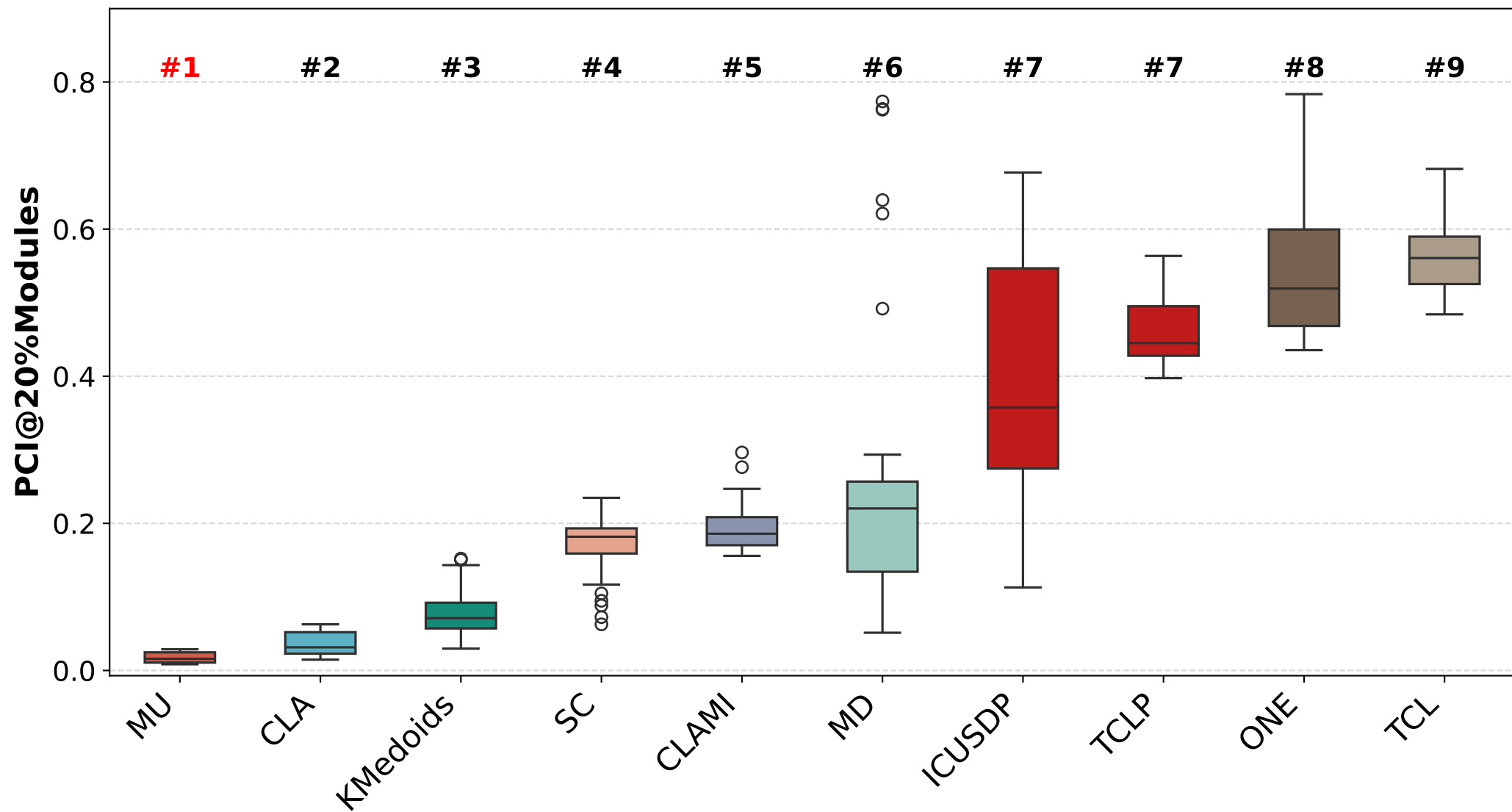
Comparison of PCI@20%Modules in Unsupervised Methods
