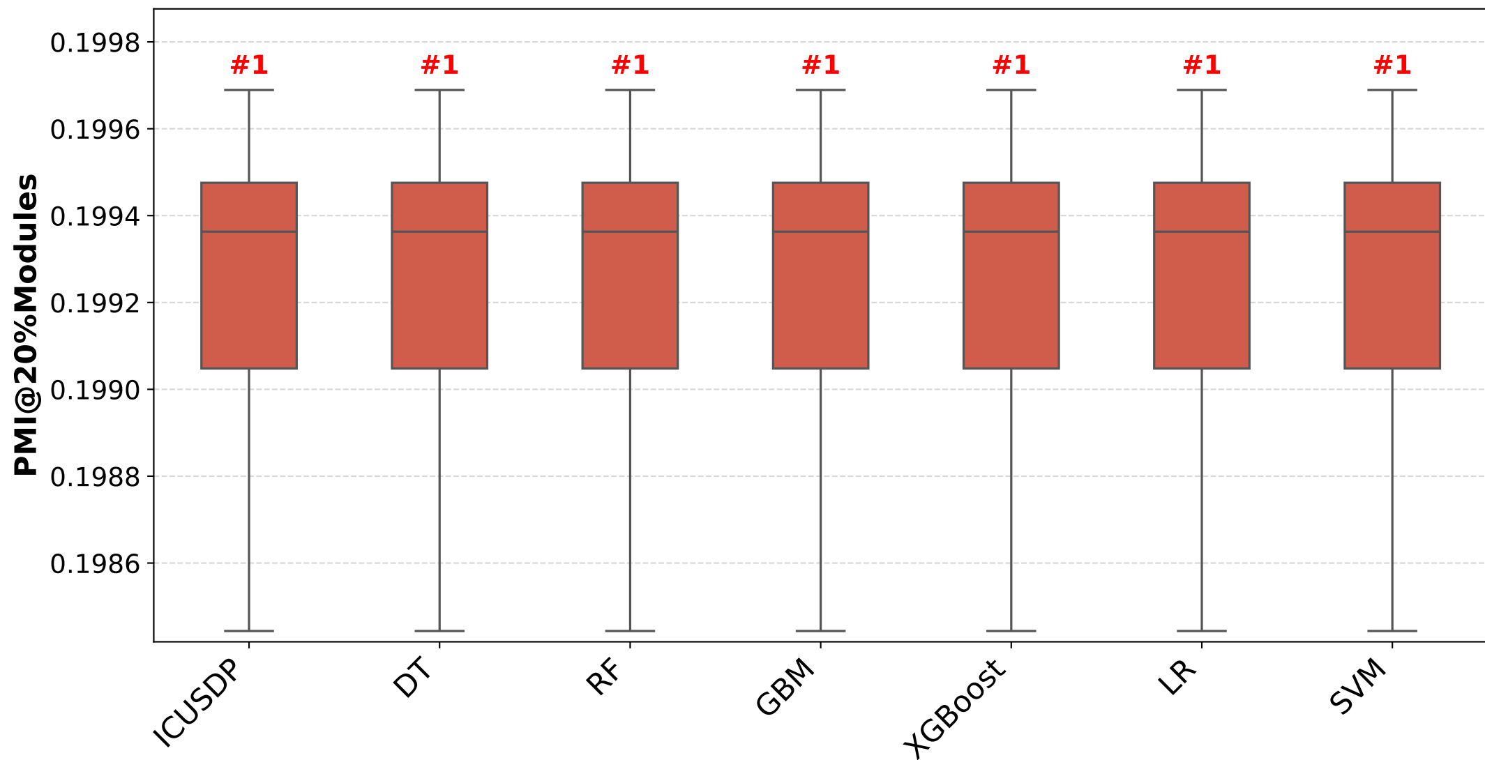
Comparison of PMI@20%Modules in Supervised Methods
