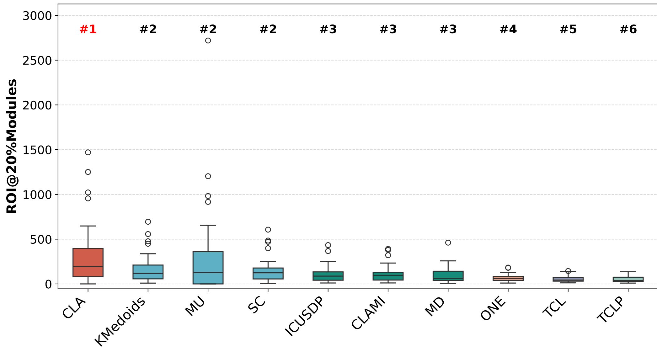
Comparison of ROI@20%Modules in Unsupervised Methods
