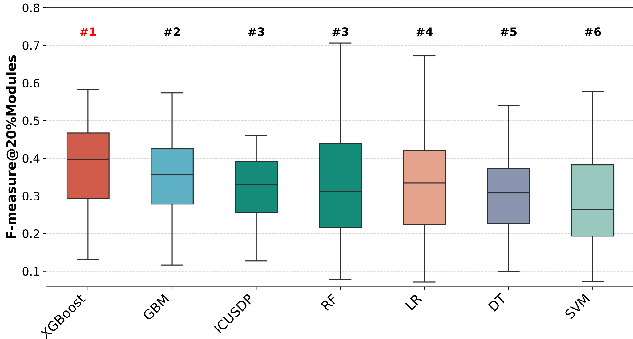
Comparison of F-measure@20%Modules in Supervised Methods
