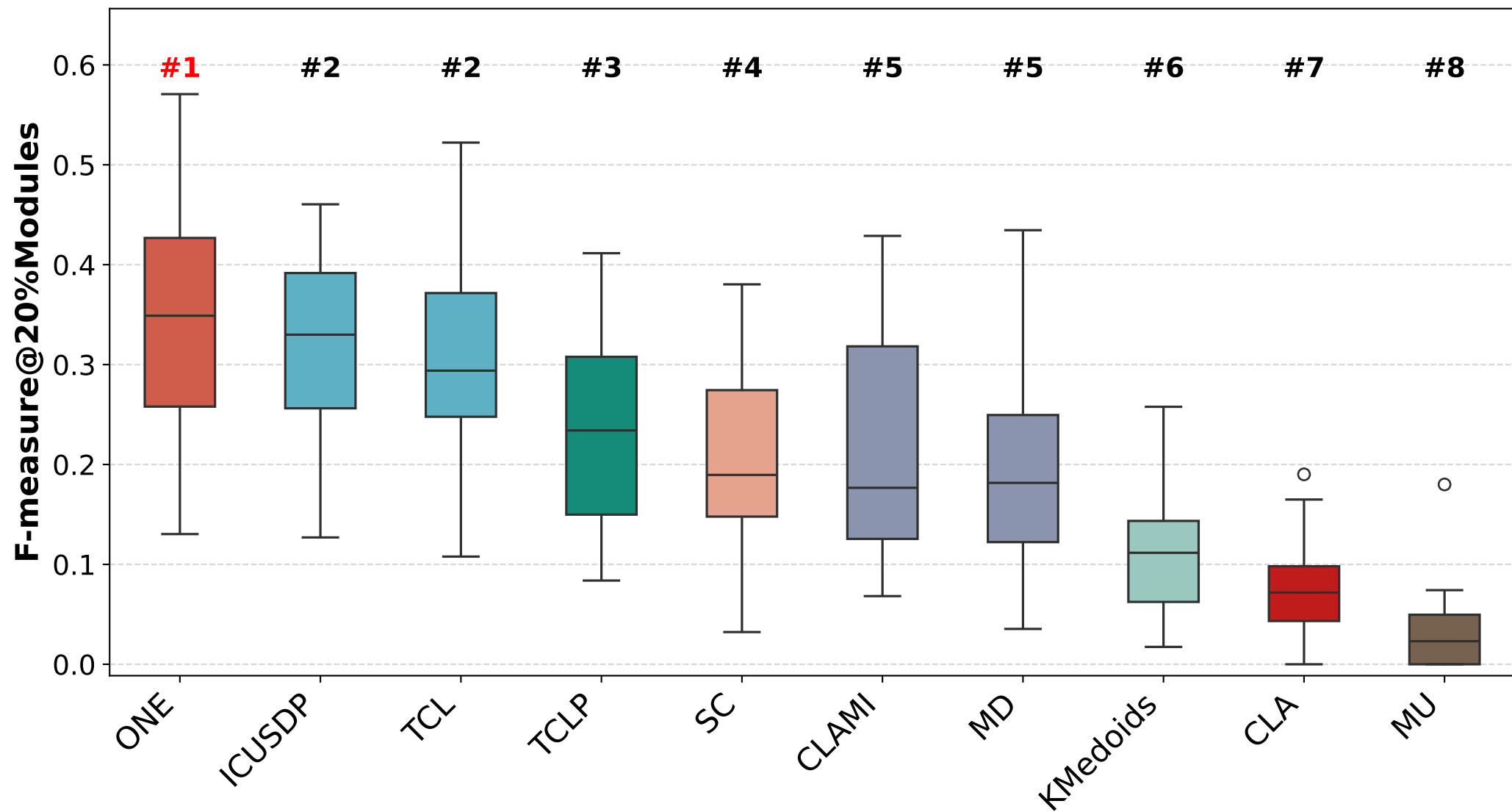
Comparison of F-measure@20%Modules in Unsupervised Methods
